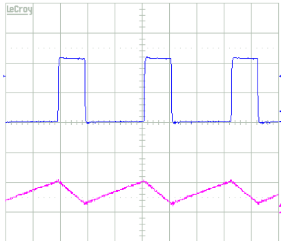
CH1:LX voltage,5V/div/DC CH4:Inductor current,500mA/div/DC Vout=10V,fosc=640kHz,L=10uH
