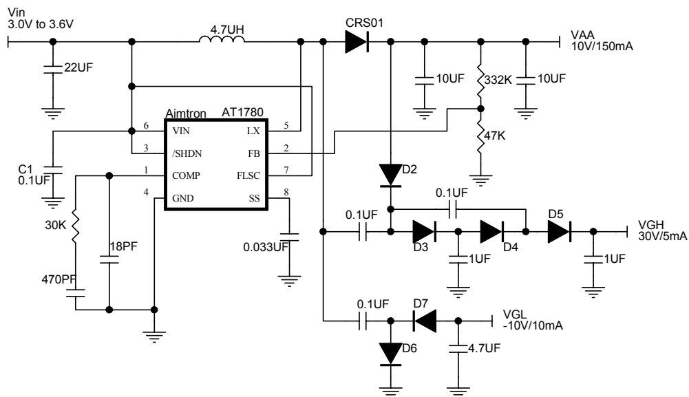
Figure 2. TFT panel power supply application circuit
