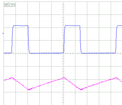
CH1:LX voltage,5V/div/DC CH4:Inductor current,500mA/div/DC Vout=10V,fosc=1.2MHz,L=4.7uH
