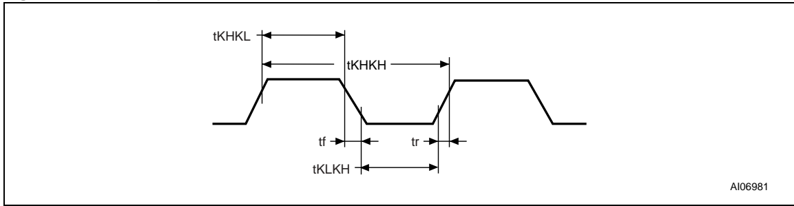
Figure 14. Clock input AC Waveform
