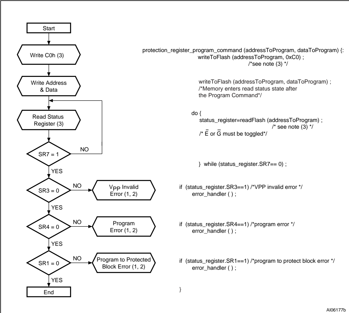
Figure 28. Protection Register Program Flowchart and Pseudo Code
