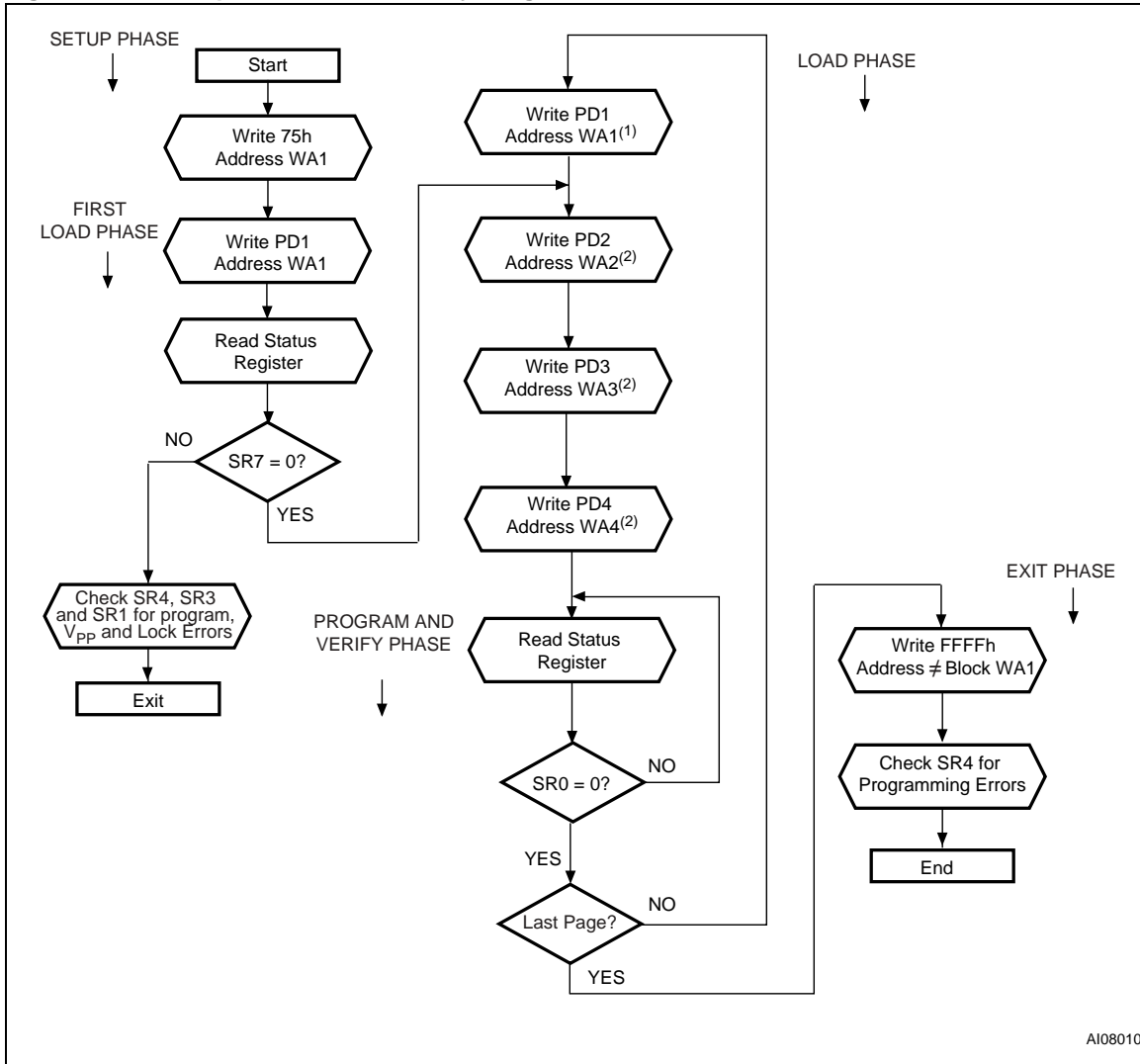
Figure 30. Quadruple Enhanced Factory Program Flowchart
