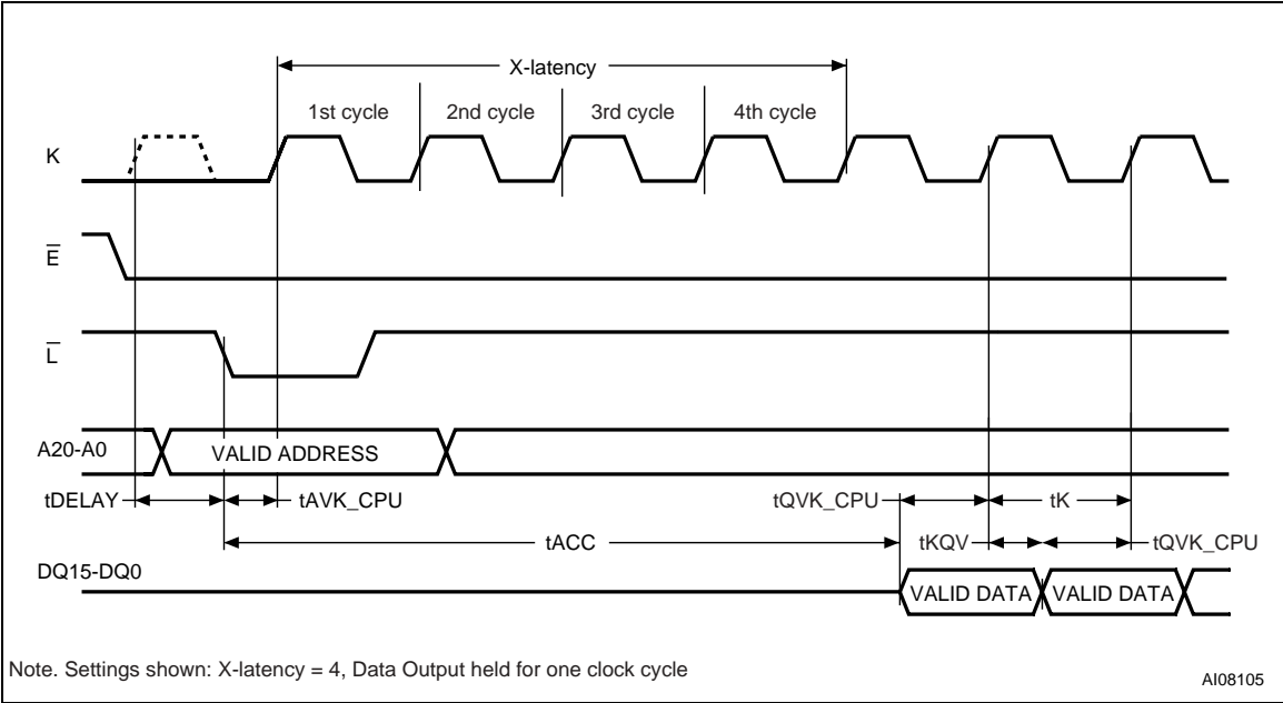
Figure 6. X-Latency and Data Output Configuration Example
