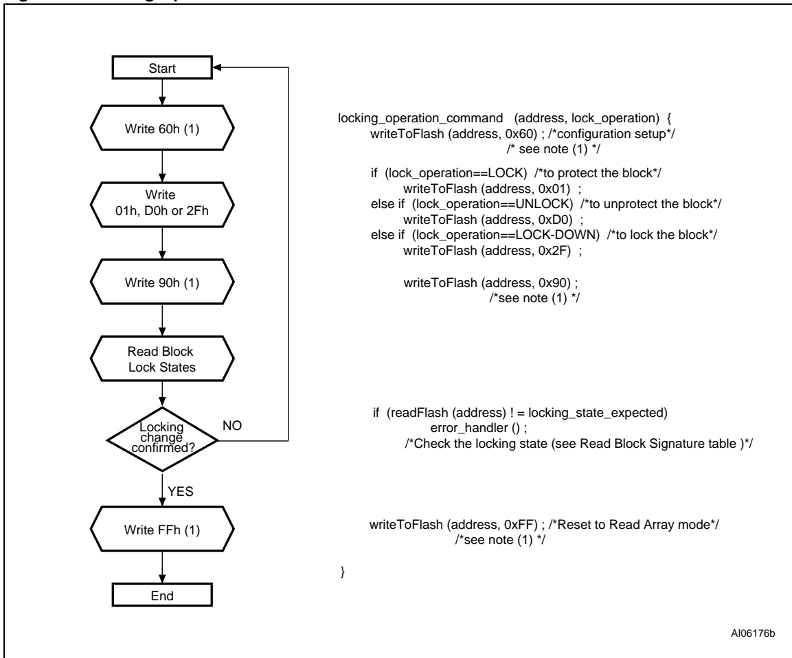
Figure 27. Locking Operations Flowchart and Pseudo Code
