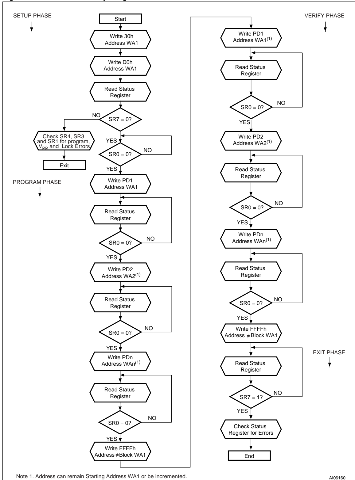
Figure 29. Enhanced Factory Program Flowchart
