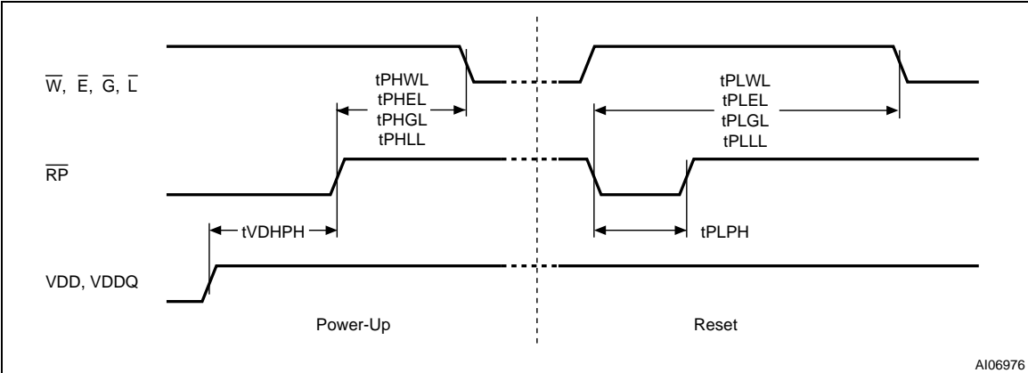
Figure 17. Reset and Power-up AC Waveforms
