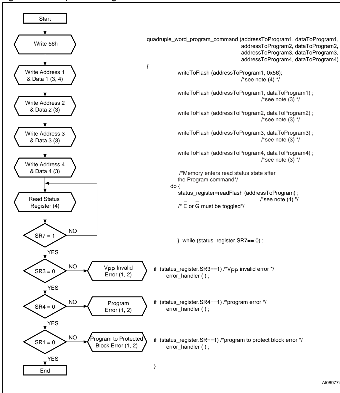
Figure 23. Quadruple Word Program Flowchart and Pseudo Code
