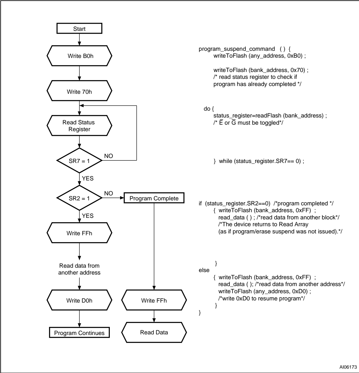
Figure 24. Program Suspend & Resume Flowchart and Pseudo Code
