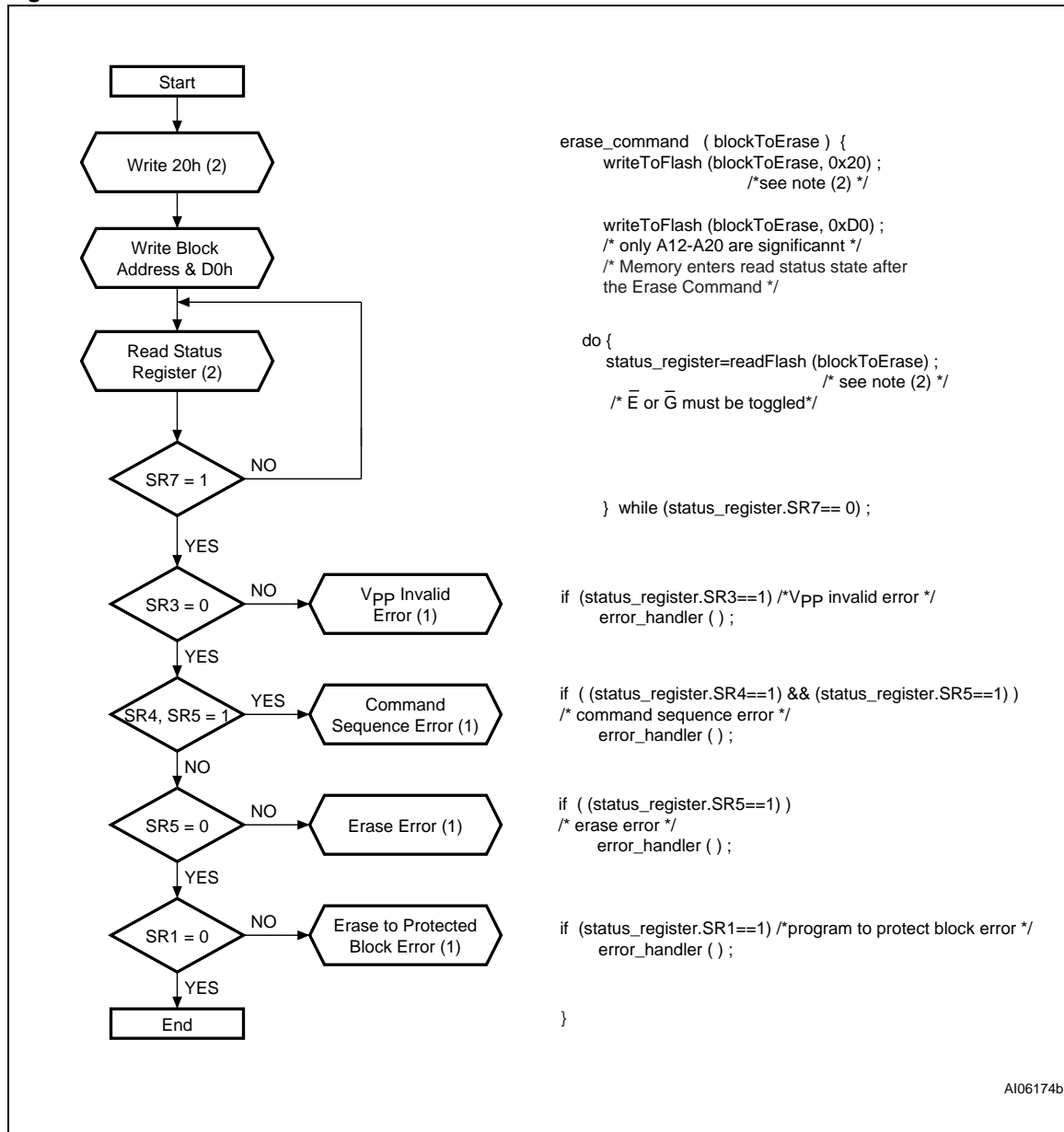
Figure 25. Block Erase Flowchart and Pseudo Code
