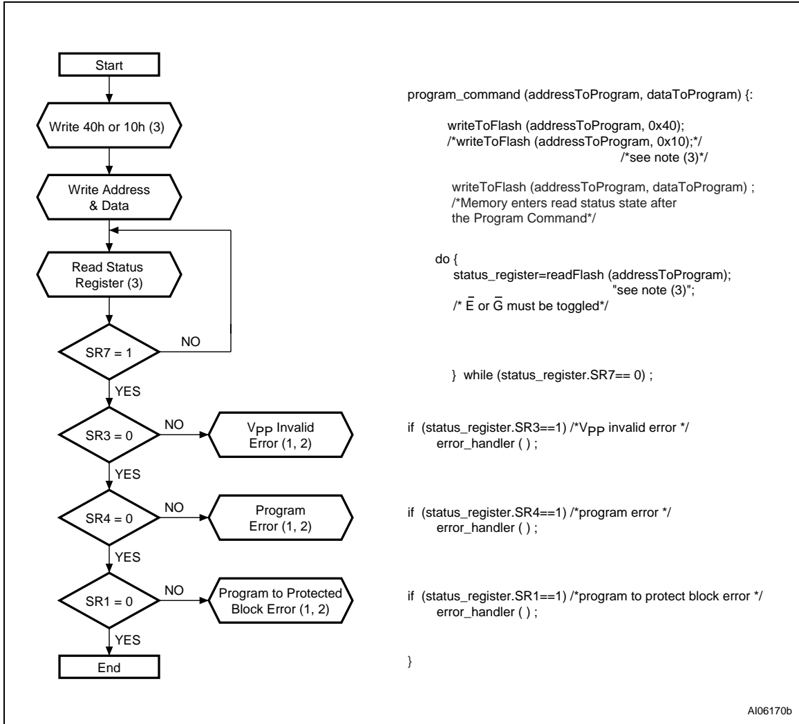
Figure 21. Program Flowchart and Pseudo Code
