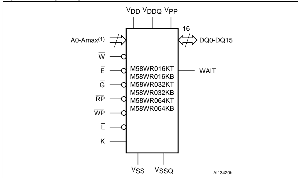
Figure 1. Logic diagram
