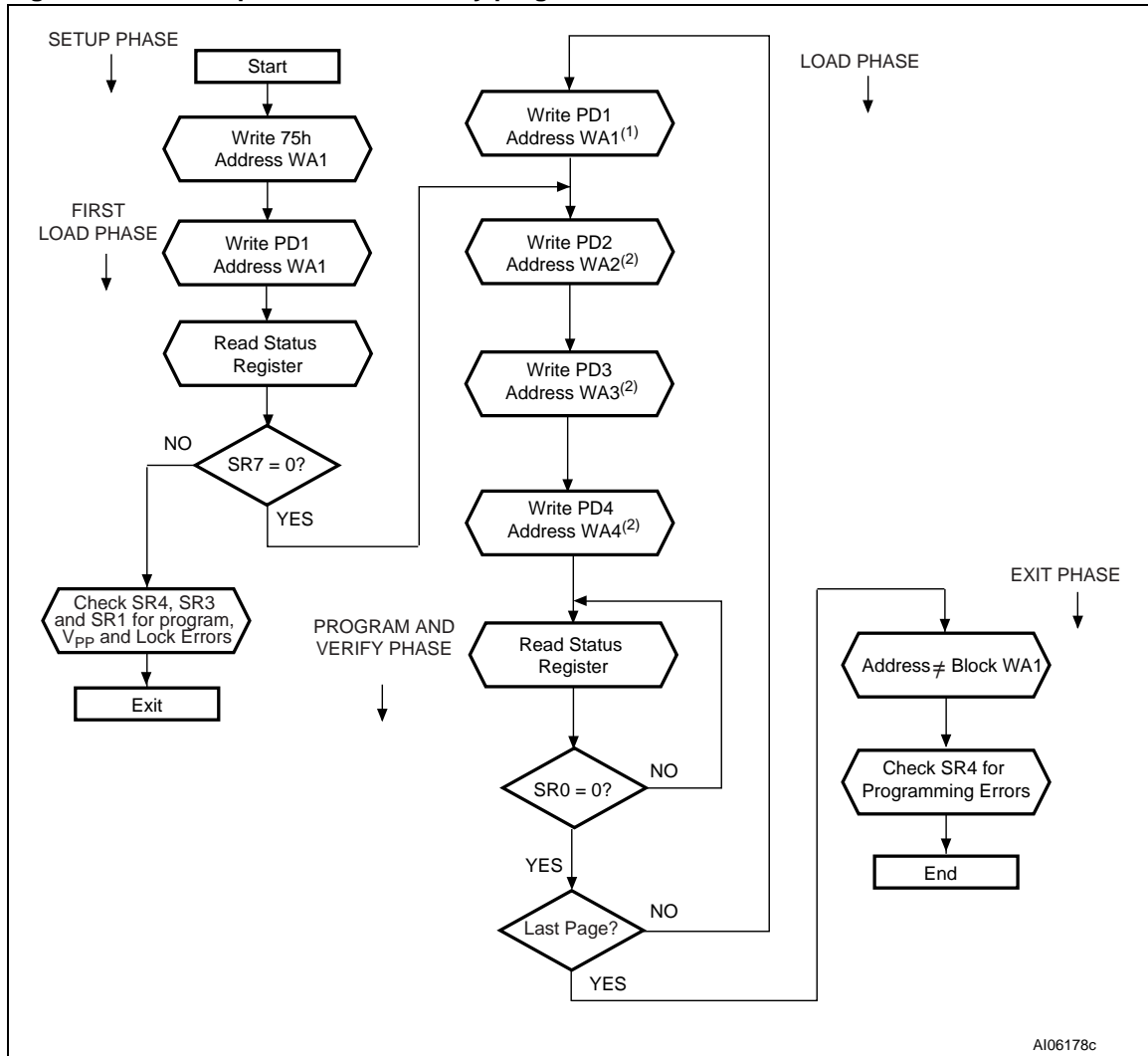
Figure 32. Quadruple enhanced factory program flowchart
