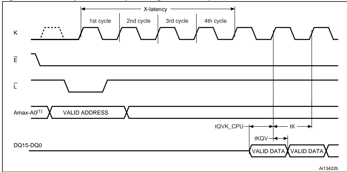
Figure 8. X-latency and data output configuration example
