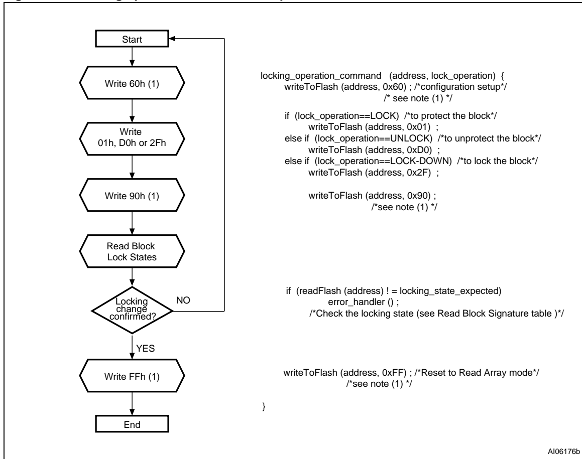
Figure 29. Locking operations flowchart and pseudo code
