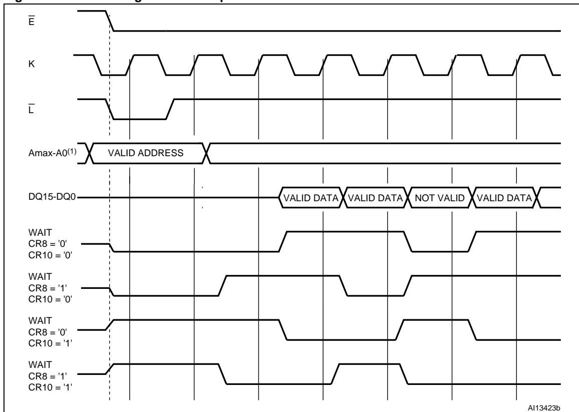
Figure 9. Wait configuration example
