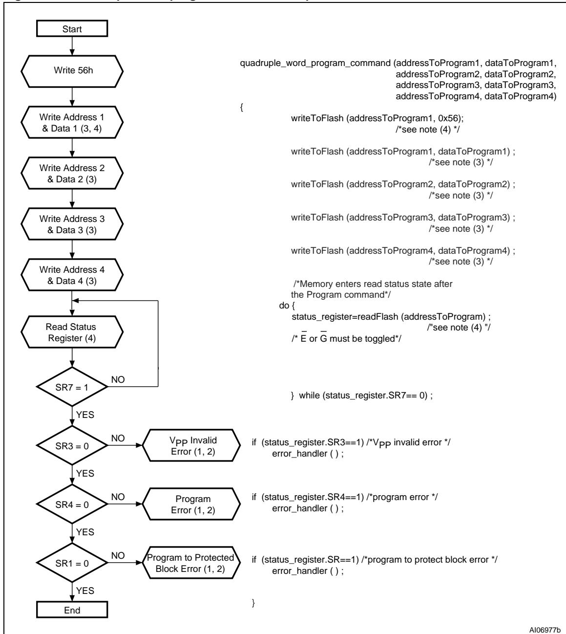
Figure 25. Quadruple word program flowchart and pseudo code
