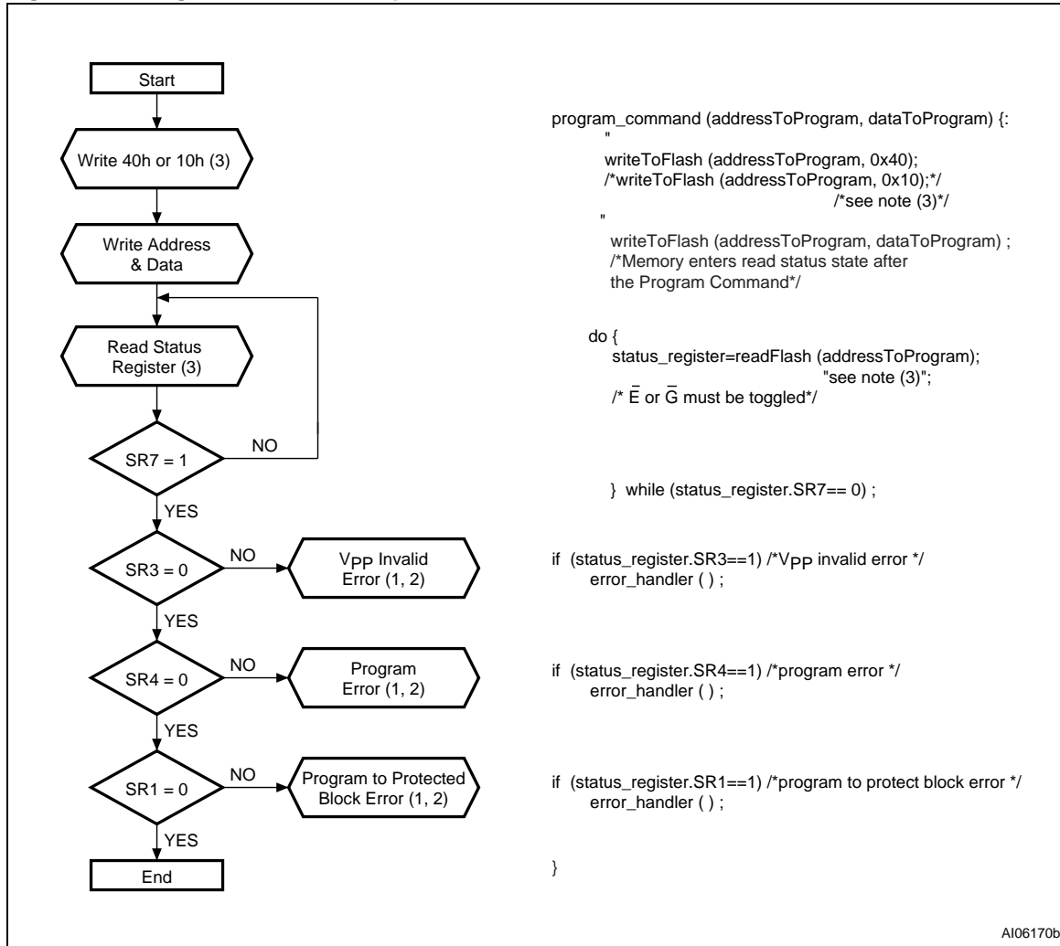
Figure 23. Program flowchart and pseudo code
