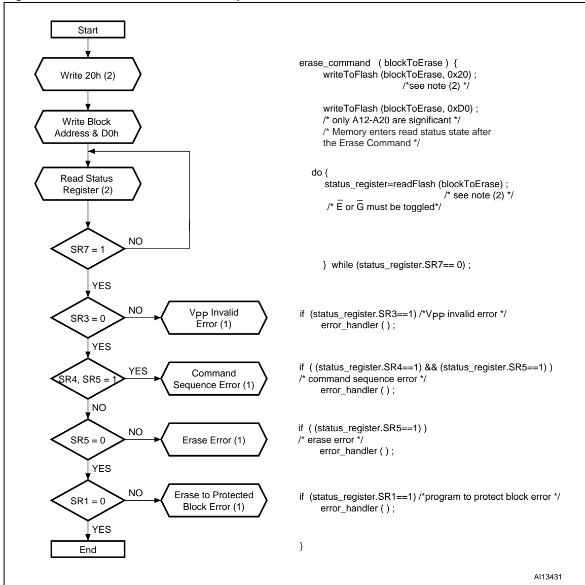
Figure 27. Block erase flowchart and pseudo code
