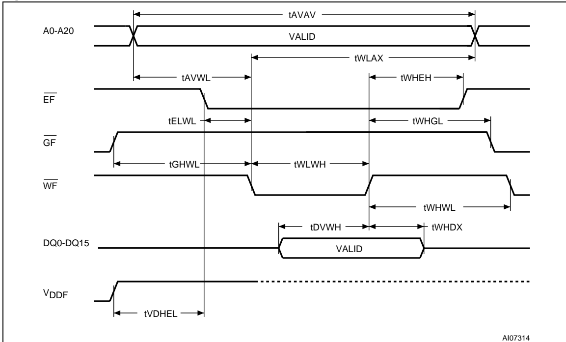
Figure 10. Flash Write AC Waveforms, Write Enable Controlled
