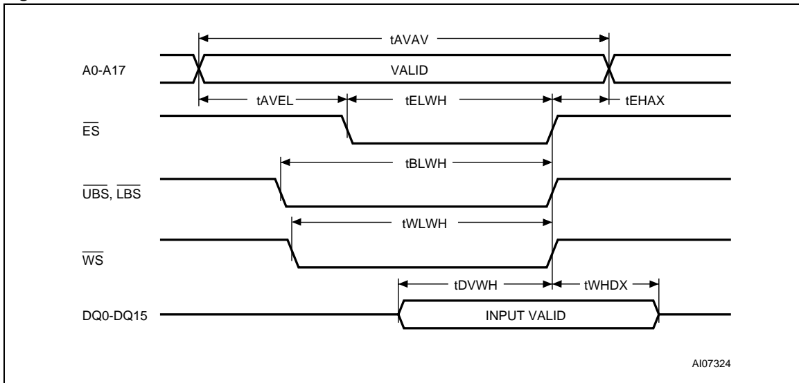
Figure 23. SRAM Write AC Waveforms, \overline{ES} Controlled
