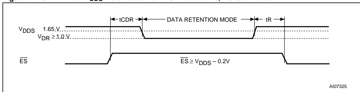
Figure 24. SRAM Low V_{DD} Data Retention AC Waveforms, \overline{ES} Controlled
