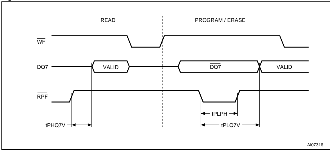
Figure 12. Flash Reset/Power-Down AC Waveform
