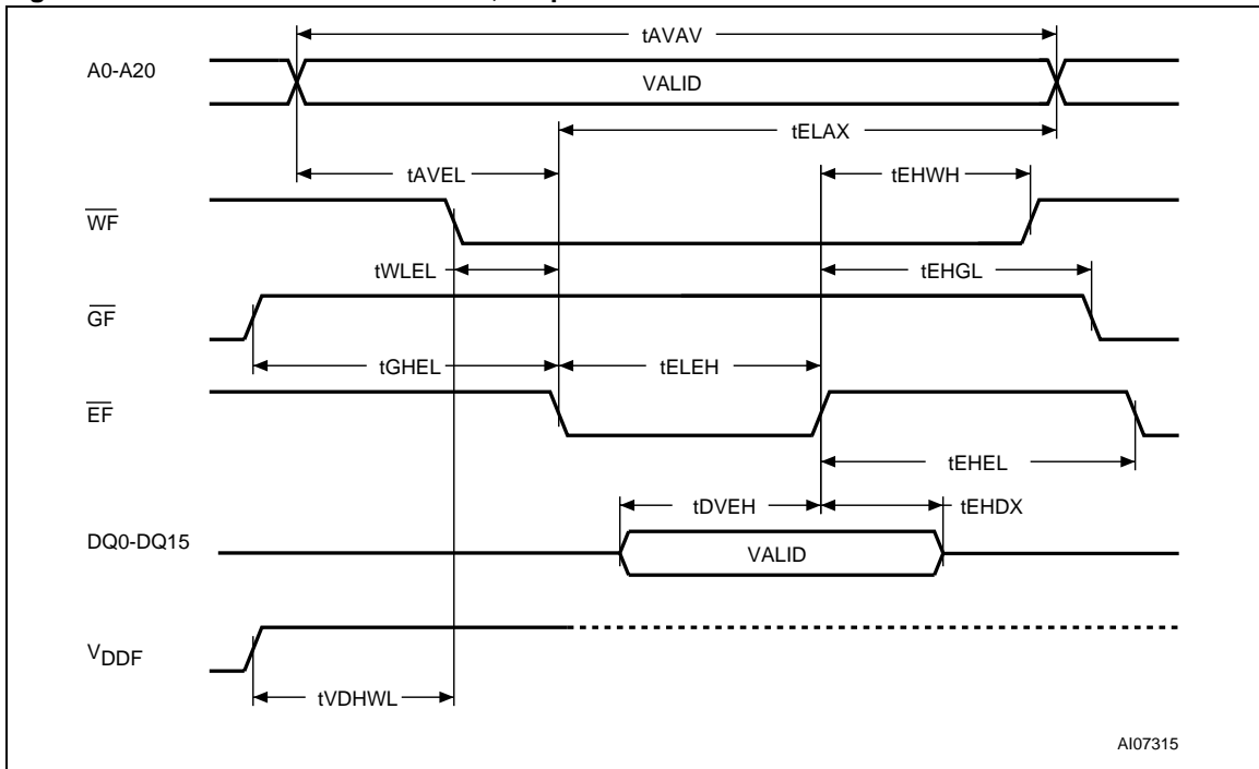
Figure 11. Flash Write AC Waveforms, Chip Enable Controlled
