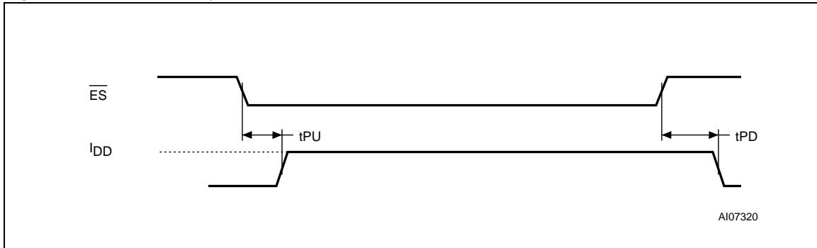
Figure 19. SRAM Standby AC Waveforms
