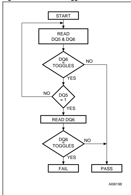
Figure 16. Flash Data Toggle Flowchart
