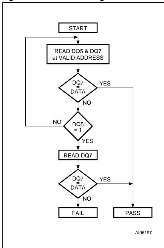
Figure 15. Flash Data Polling Flowchart
