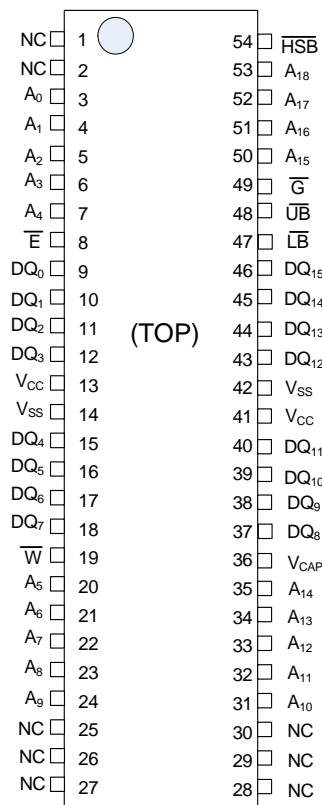
54-Pin TSOP-II
