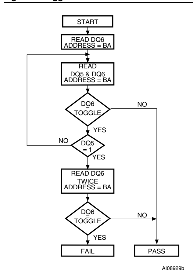
Figure 8. Toggle Flowchart
