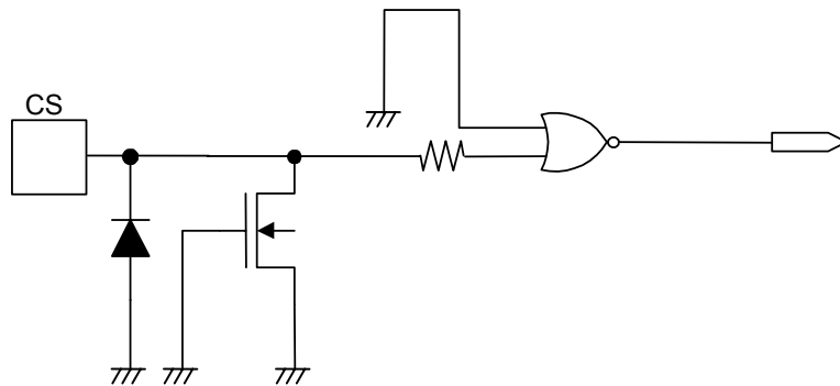
Figure 23 CS Pin
