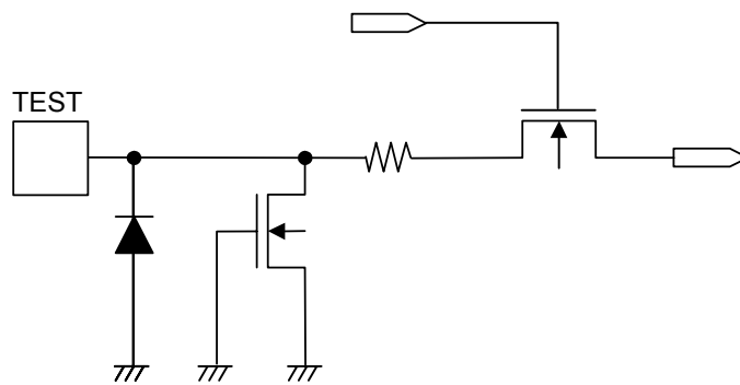
Figure 25 TEST Pin
