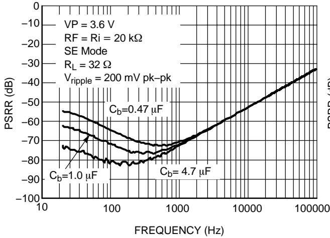
Figure 20. PSRR vs. C_b (SE Mode) @ V_P = 3.6\text{ V}
