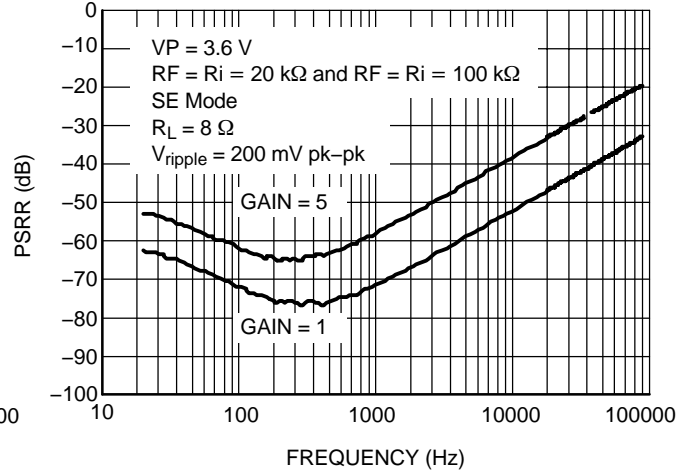
Figure 21. PSRR vs. Gain (SE Mode) @ V_P = 3.6\text{ V}
