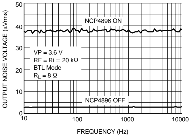
Figure 22. Output Noise Voltage (BTL Mode) @ V_P = 3.6\text{ V}
