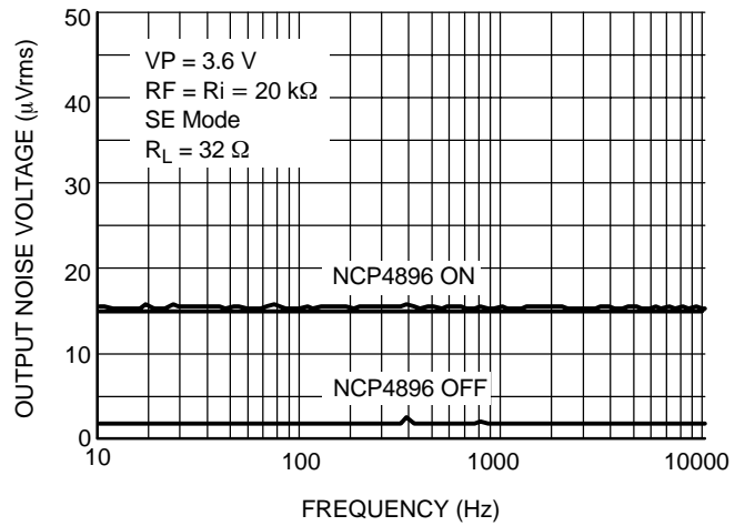
Figure 23. Output Noise Voltage (SE Mode) @ V_P = 3.6\text{ V}
