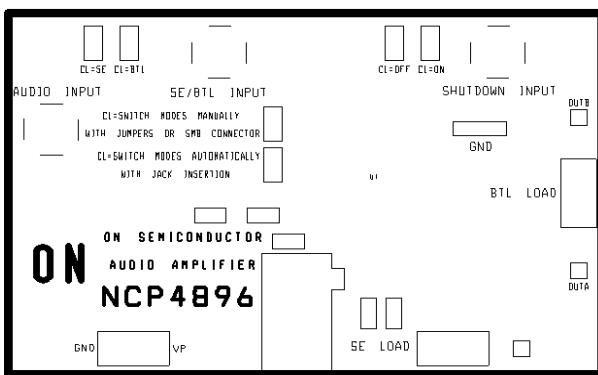
Silkscreen Layer
