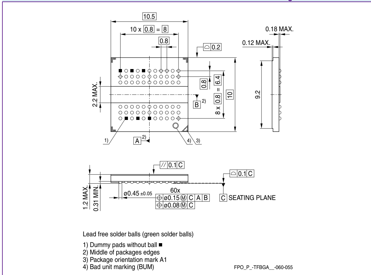
FIGURE 11 Package Outline P-TFBGA-60
