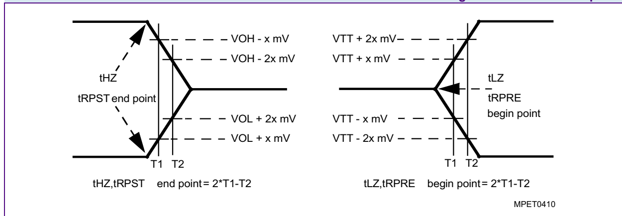
Method for Calculating Transitions and Endpoint
