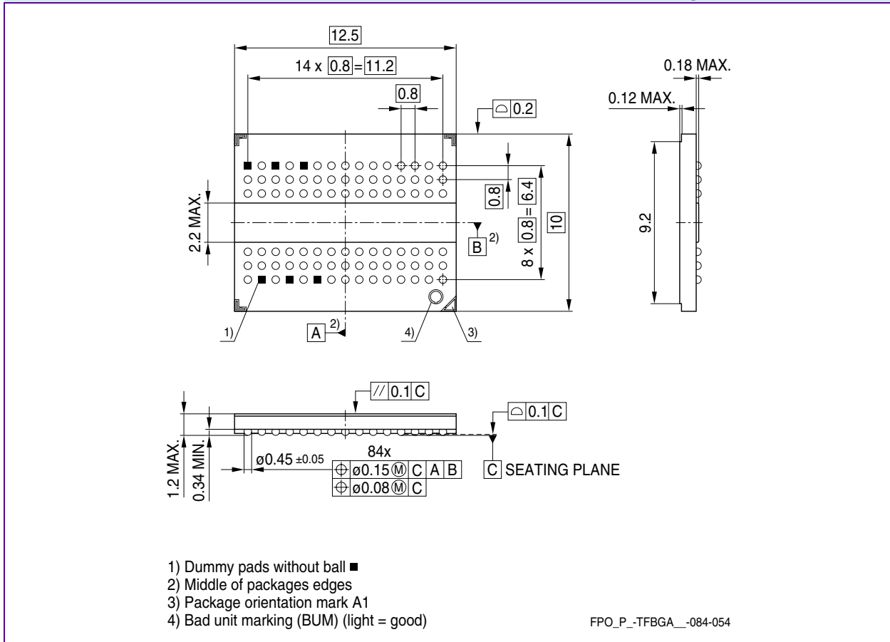
FIGURE 13 Package Outline P-TFBGA-84
