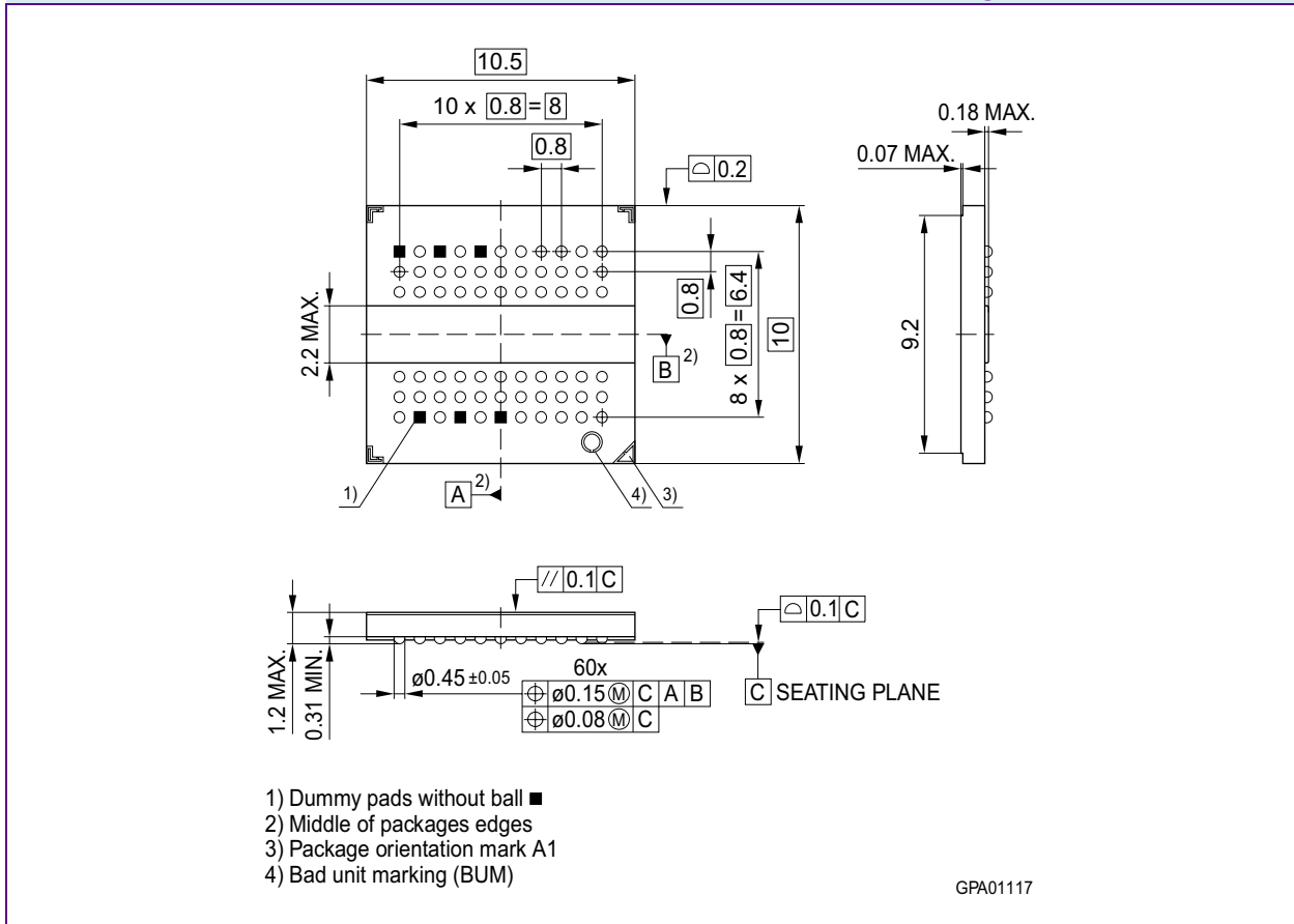
FIGURE 12 Package Outline PG-TFBGA-60
