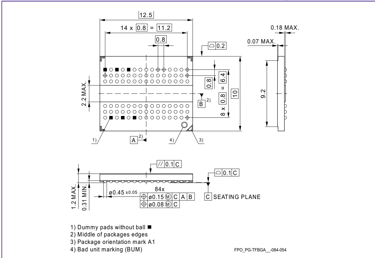
FIGURE 14 Package Outline PG-TFBGA-84
