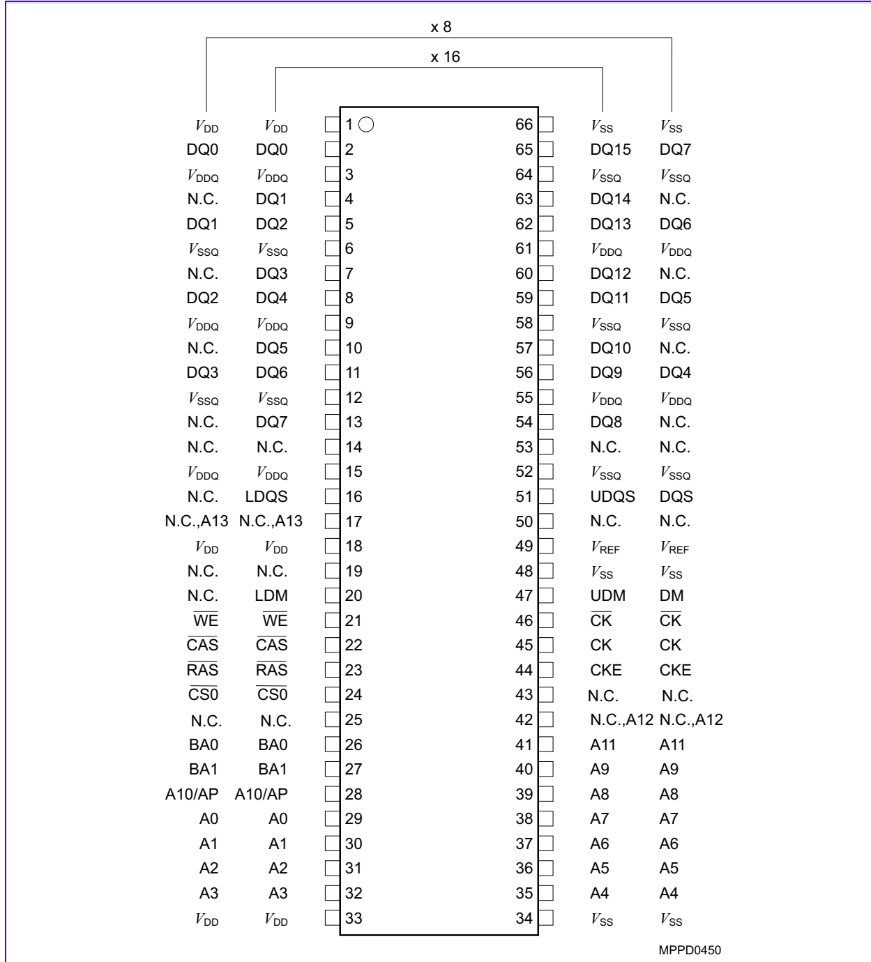
FIGURE 3 Chip Configuration PG-TSOPII-66
