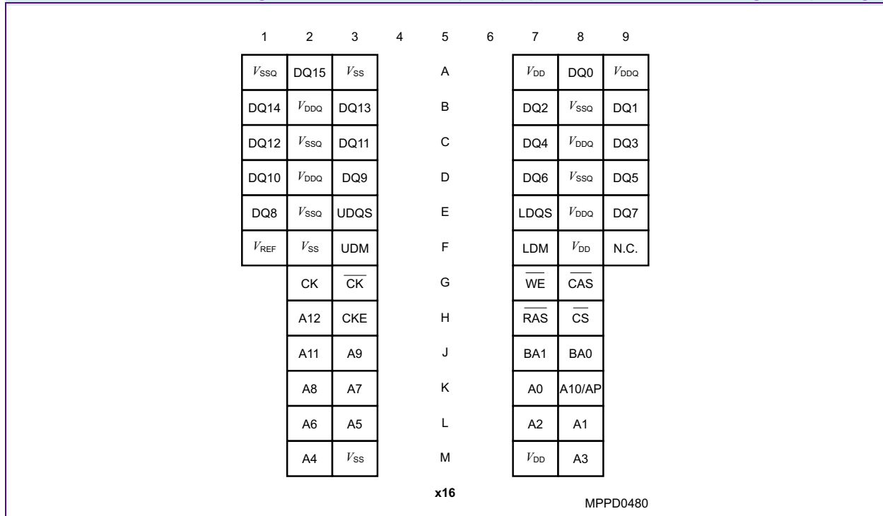
Pin Configuration PG-TFBGA-60 ( x16 )Top View, see the balls through the package
