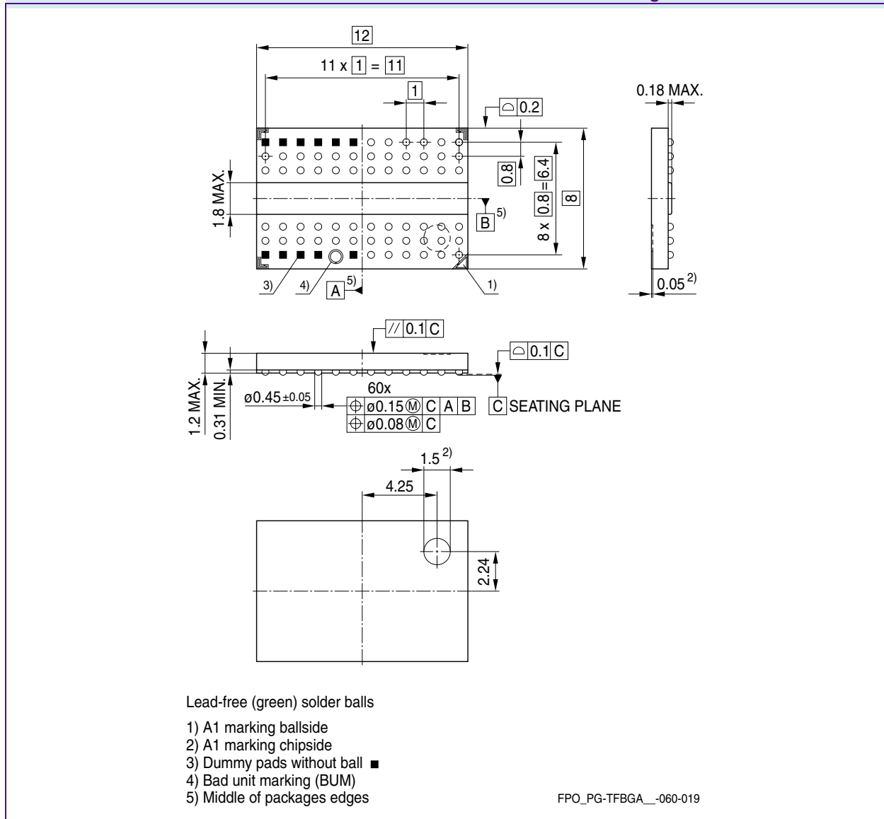
FIGURE 6 Package Outline of PG-TFBGA-60
