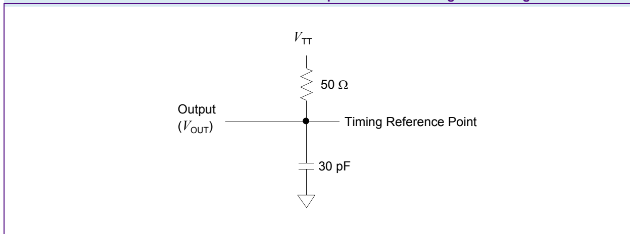
FIGURE 4 AC Output Load Circuit Diagram / Timing Reference Load
