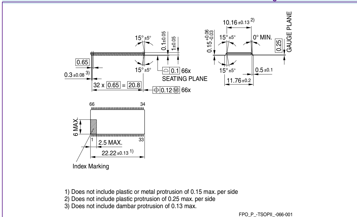
FIGURE 5 Package Outline PG-TSOPII-66
