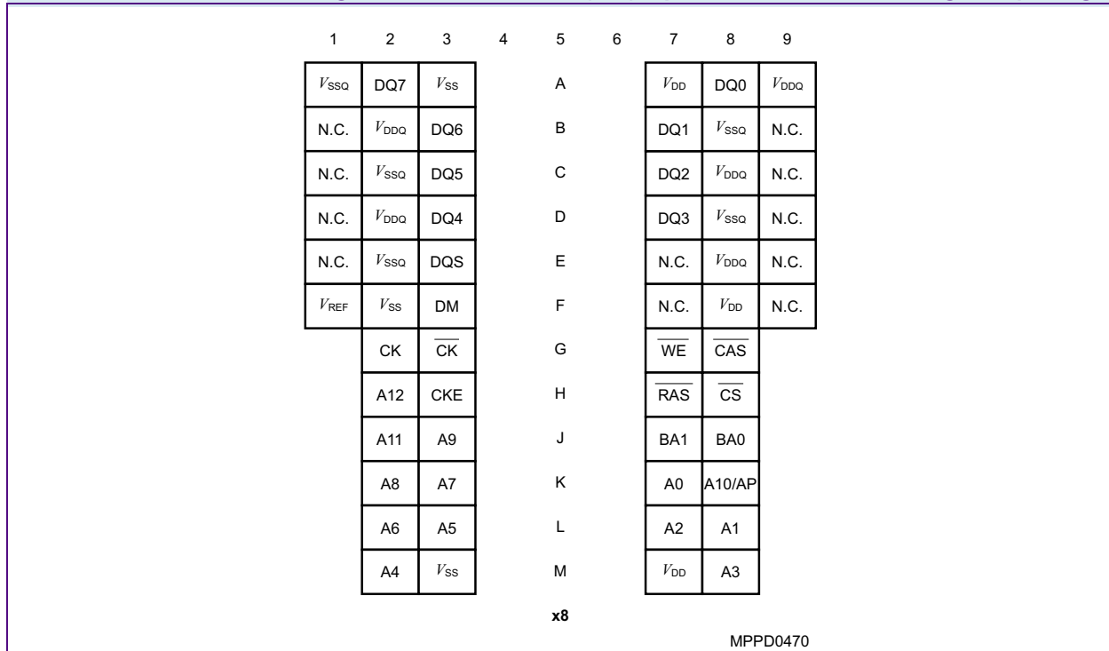
Pin Configuration PG-TFBGA-60 ( x8 )Top View, see the balls through the package
