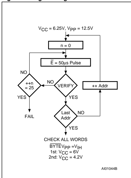
Figure 9. Programming Flowchart
