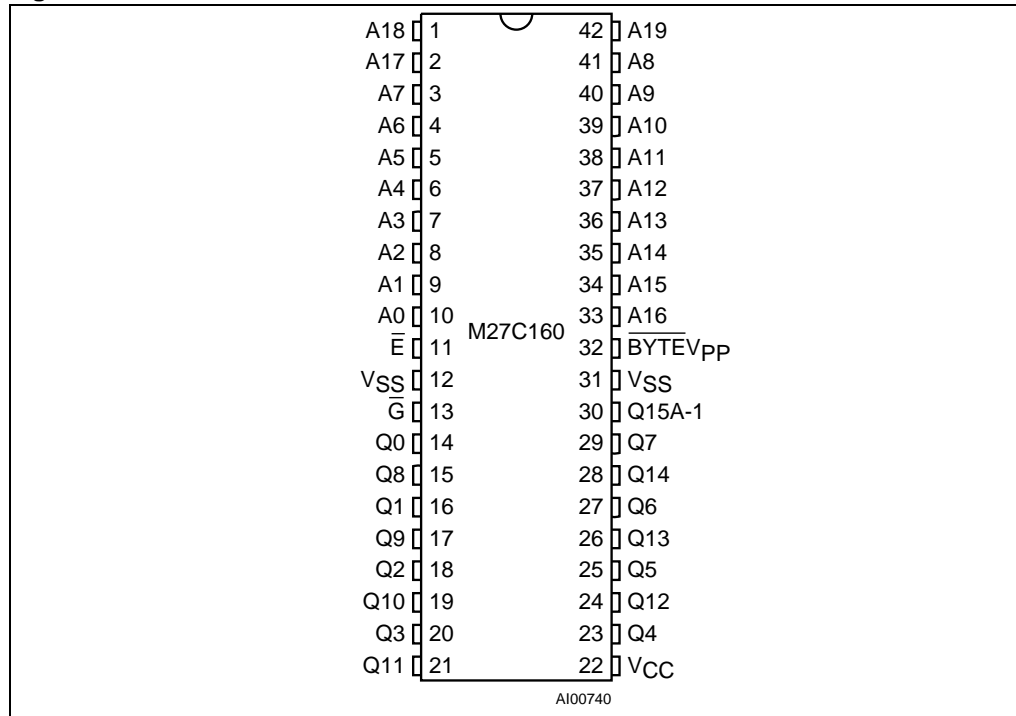
Figure 3. DIP Connections
