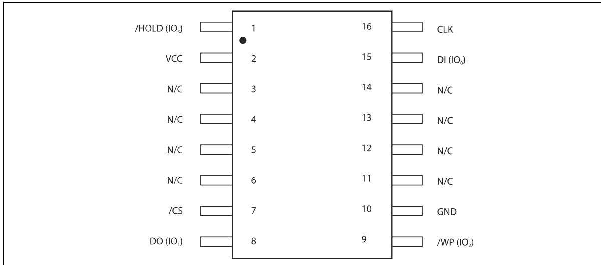
Figure 1c. W25Q16BV Pin Assignments, 16-pin SOIC 300-mil (Package Code SF)
