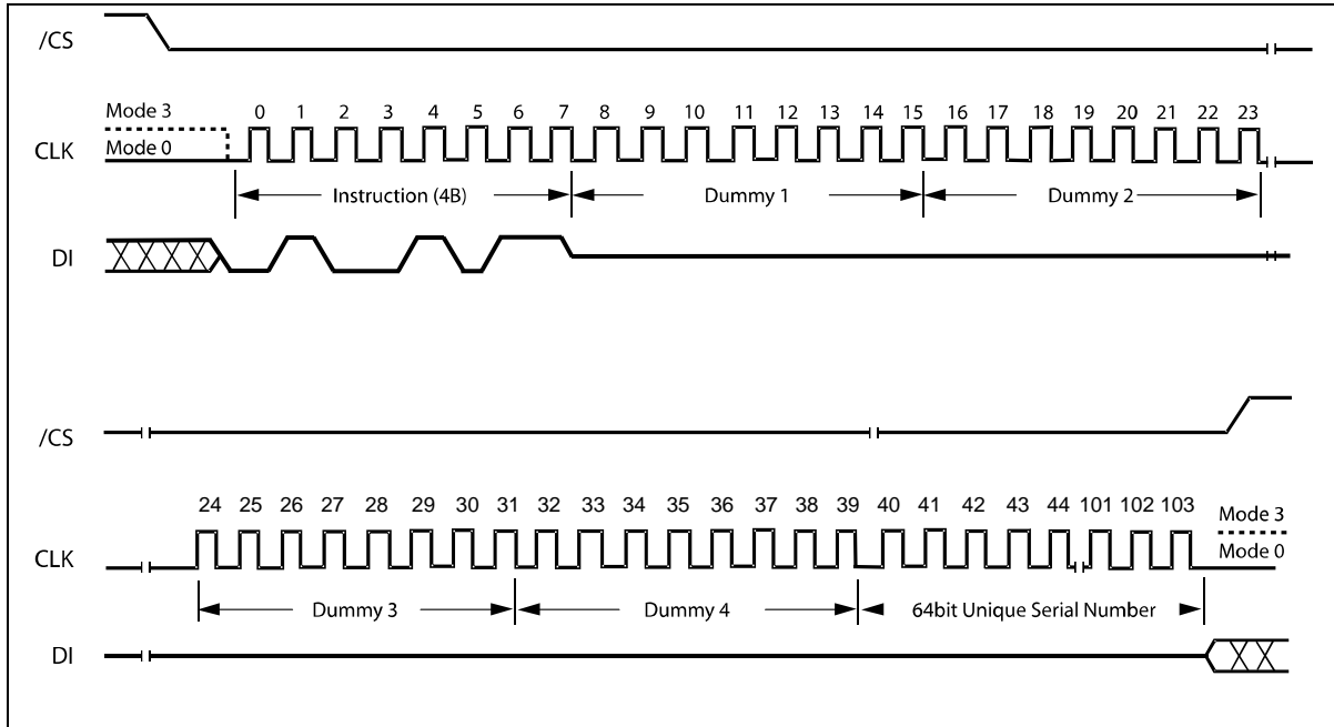
Figure 29. Read Unique ID Number Instruction Sequence Diagram
