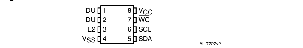
Figure 2. SO8 connections
