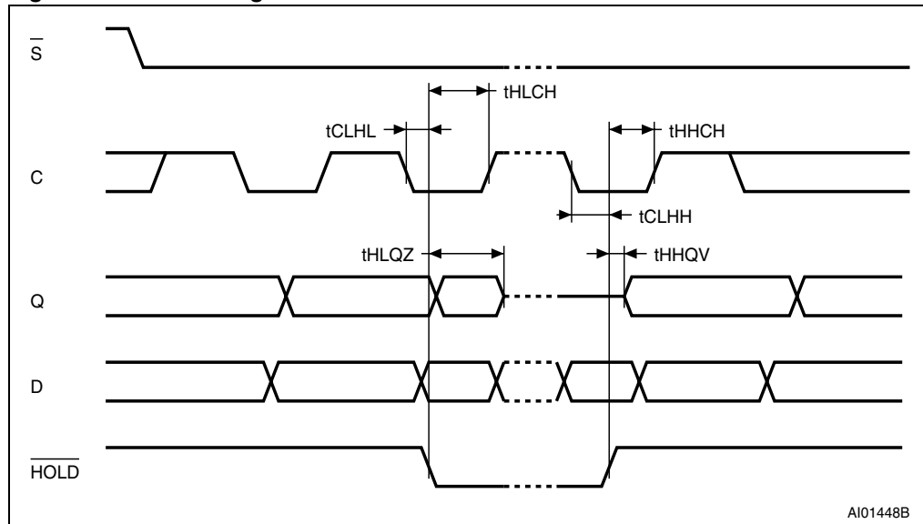
Figure 16. Hold timing
