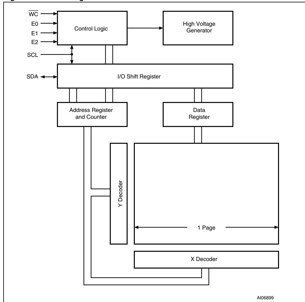
Figure 8. Block diagram
