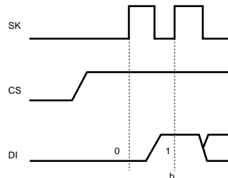
Fig. 17 Normal operation timing
