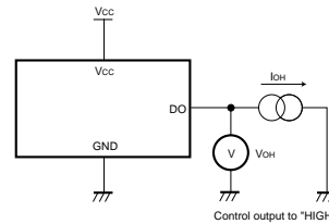
Fig.4 "HIGH" output voltage circuit
