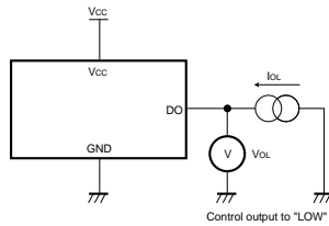
Fig.3 "LOW" output voltage circuit
