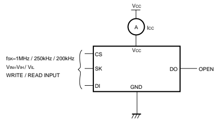
Fig.7 Supply current circuit
