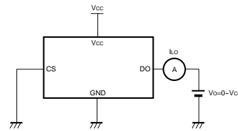
Fig.6 Output leak current circuit
