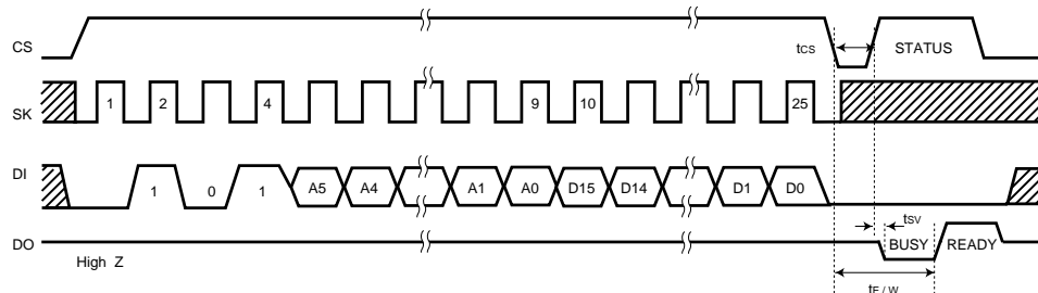
Fig.12 Write cycle timing (WRITE)
