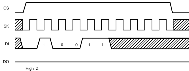
Fig.11 Write enable cycle timing
