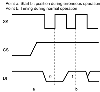
Fig. 16 Erroneous operation timing
