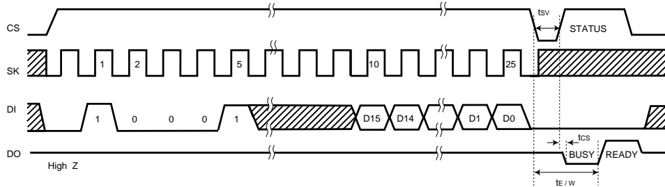
Fig.13 Write all address cycle timing. (WRAL)
