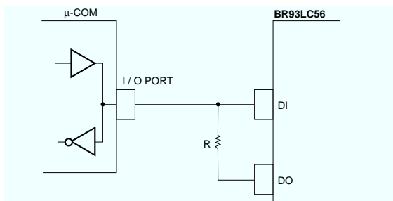
Fig. 11 Common connections for the DI and DO control line
