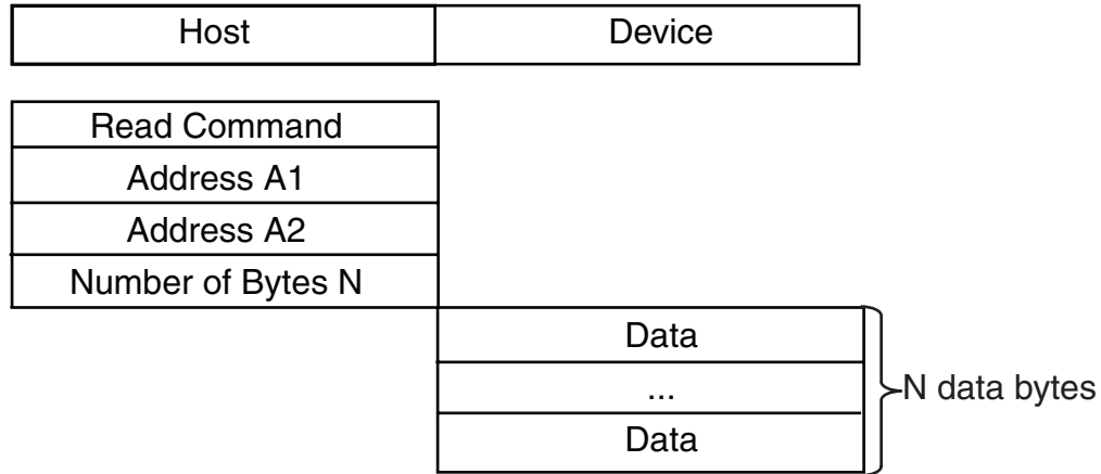
Figure 8-3. Read User Zone Command Functional Description
