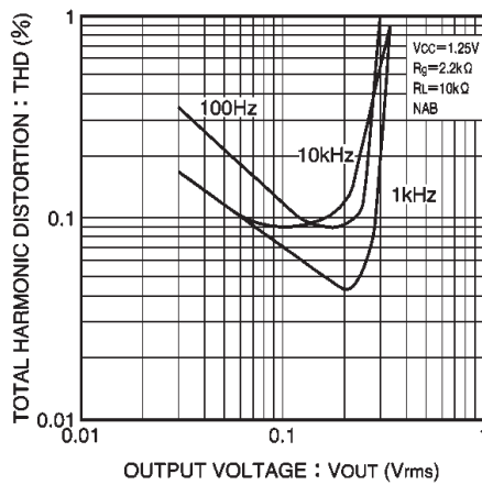
Fig. 12 Total harmonic distortion vs. output voltage
