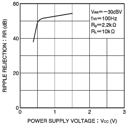
Fig. 8 Ripple rejection ratio vs. power supply voltage
