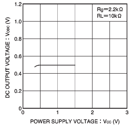
Fig. 7 DC output voltage vs. power supply voltage
