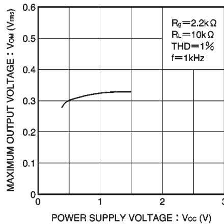
Fig. 6 Maximum output voltage vs. power supply voltage
