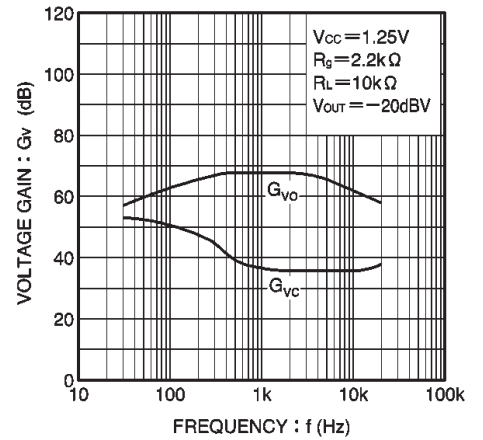
Fig. 10 Voltage gain vs. frequency
