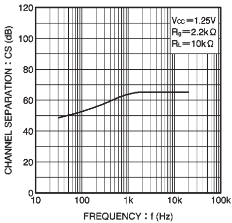
Fig. 11 Crosstalk vs. frequency
