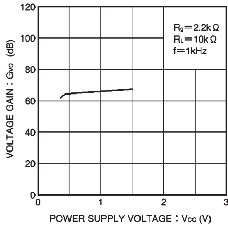
Fig. 9 Voltage gain vs. power supply voltage
