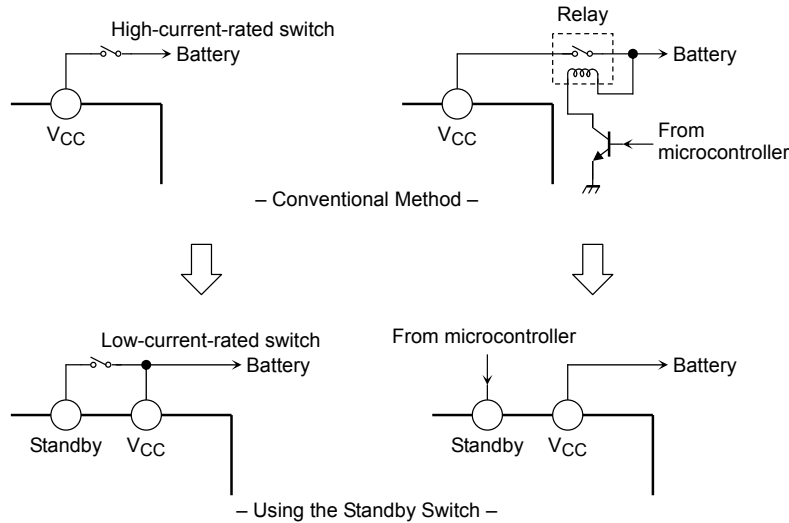
Figure 2 Standby Switch
