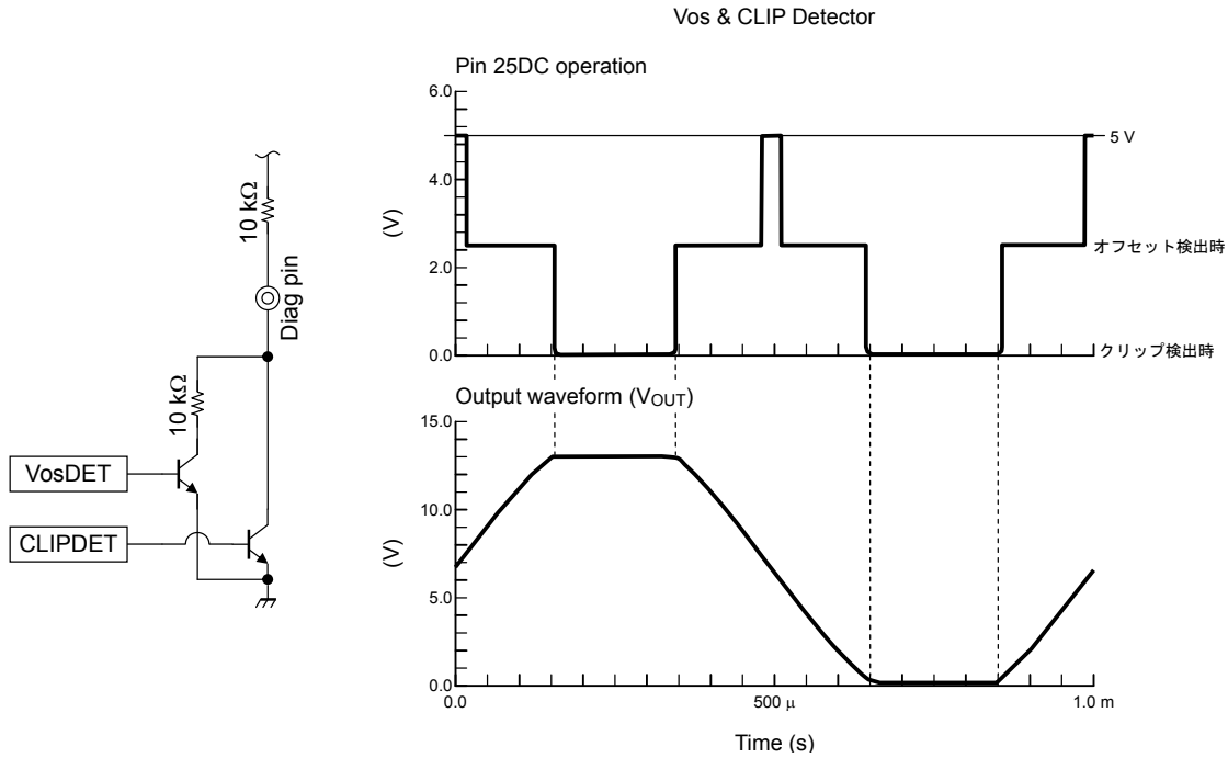
Figure 6 Open-Collector Output of Pin 25
