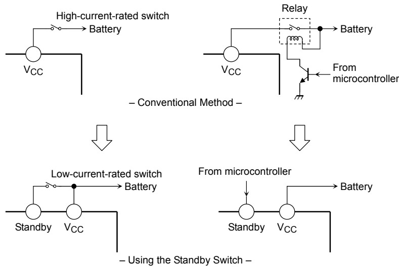
Figure 2 Standby Switch
