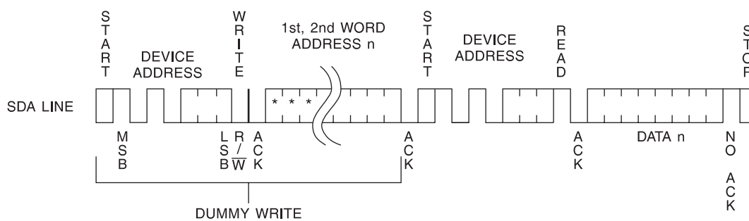
Figure 12-5. Random Read
