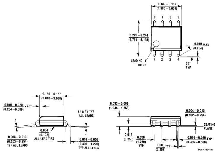
8-Pin Small Outline Package Order Number LM6311IM or LM6311MX NS Package Number M08A
