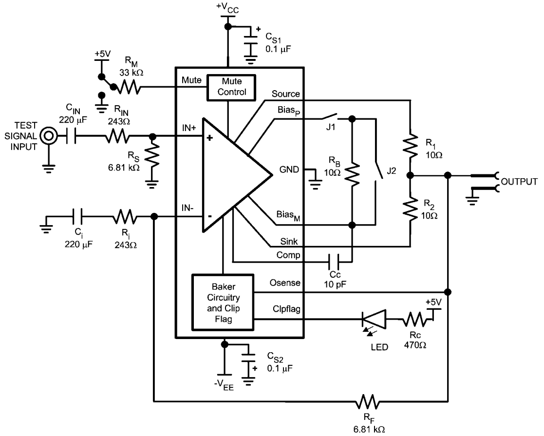
FIGURE 4. LME49810 Test demo board schematic
