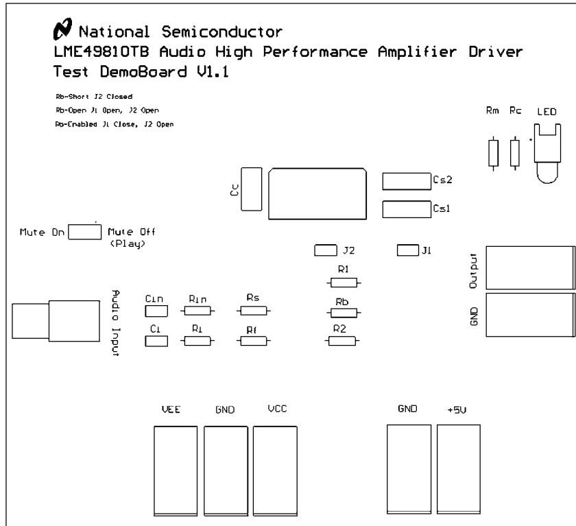
Silkscreen Layer
