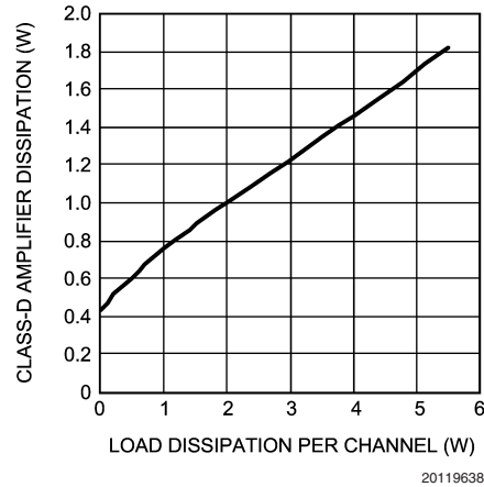
Class-D Amplifier Dissipation vs Load Dissipation Per Channel, V_{DD} = 15V , R_L = 8\Omega (both channels driven and measured)
