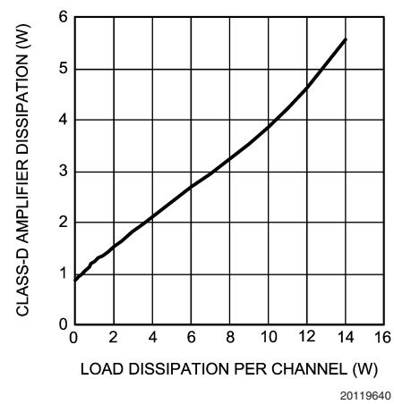
Class-D Amplifier Dissipation vs Load Dissipation Per Channel, V_{DD} = 15V , R_L = 8\Omega (both channels driven and measured)
