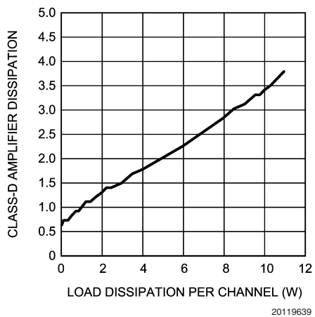
Class-D Amplifier Dissipation vs Load Dissipation Per Channel, V_{DD} = 12V , R_L = 8\Omega (both channels driven and measured)
