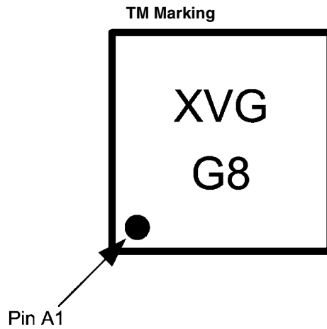
20159949 Top View X - Date Code V - Die Traceability G - Boomer Family G8 - LM4995TM
