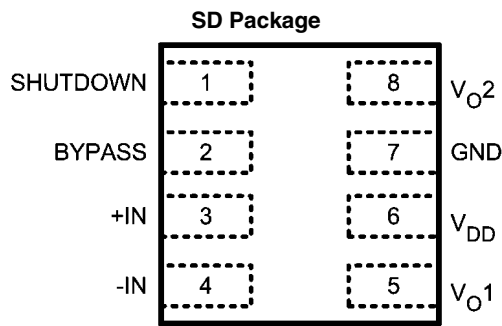
20159957 Top View Order Number LM4995SD See NS Package Number SDA08A
