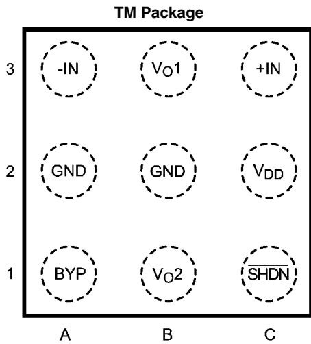
20159903 Top View Order Number LM4995TM See NS Package Number TMD09AAA
