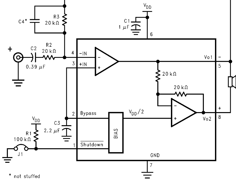
FIGURE 4. REFERENCE DESIGN BOARD SCHEMATIC
