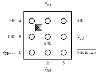
Top View Order Number LM4990ITL, LM4990ITLX See NS Package Number TLA09ZZA
