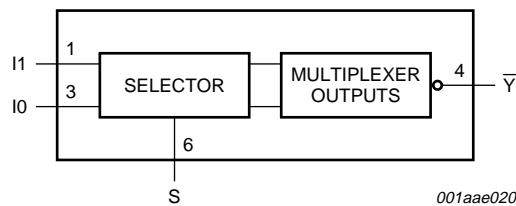
Fig 2. IEC logic symbol
