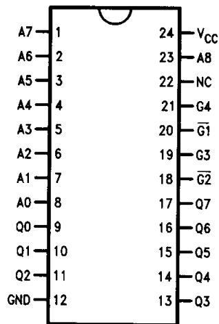
Dual-In-Line-Package
