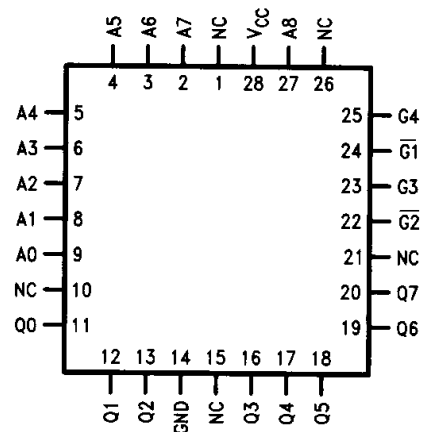
Plastic Leaded Chip Carrier (PLCC)
