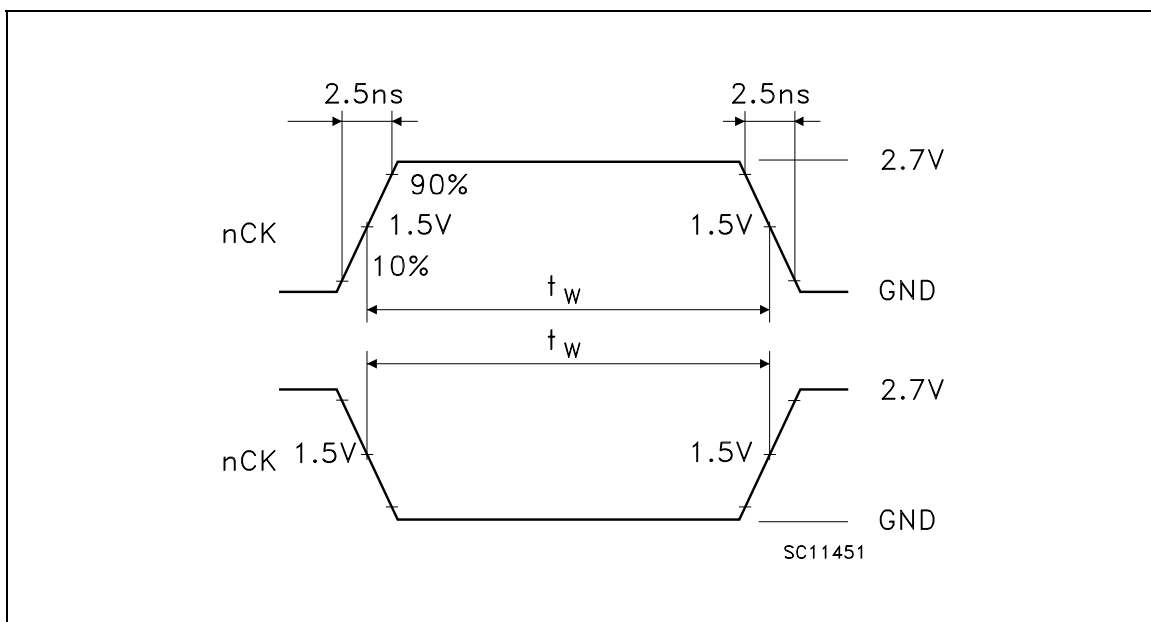
WAVEFORM 3 : PULSE WIDTH (f=1MHz; 50% duty cycle)
