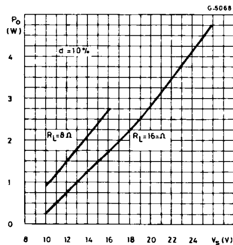
Figure 12 : Output Power vs. Supply Voltage.
