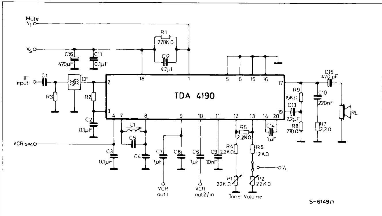
Figure 16 : Application Circuit.
