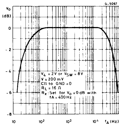
Figure 11 : Audio Amplifier Frequency Response.
