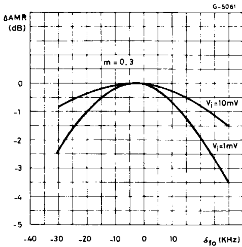
Figure 5 : \Delta AMR vs. Tuning Frequency Change
