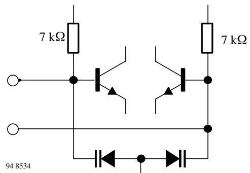
Figure 16. VCO (Pin 20-21)
