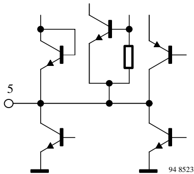
Figure 7. SIF-AGC time constant (Pin 5)
