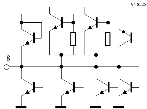
Figure 9. VIF-AGC time constant (Pin 8)
