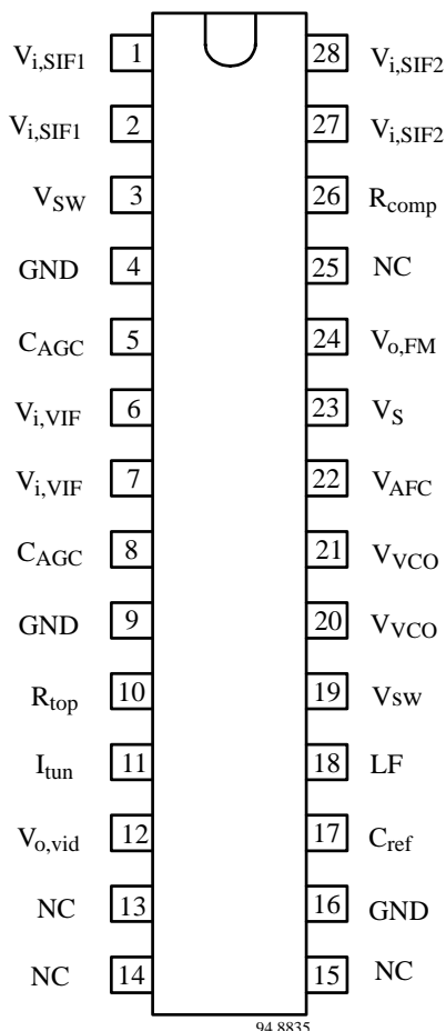
Figure 2. Pinning
