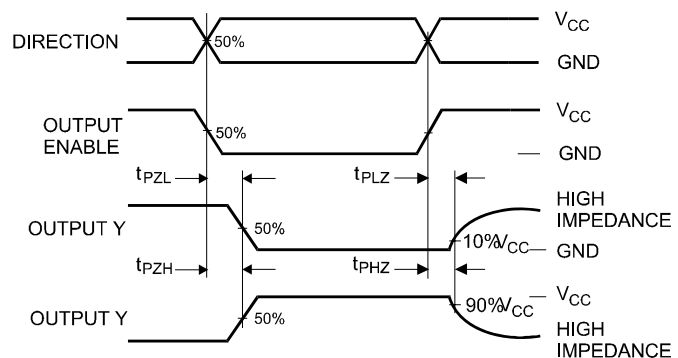
Figure 2. Switching Waveforms
