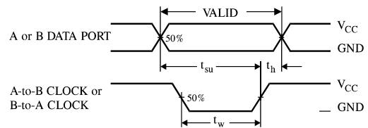
Figure 7. Switching Waveforms
