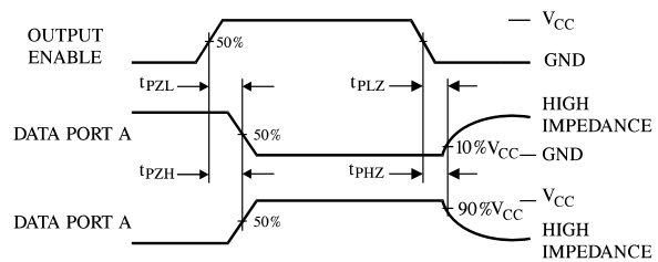
Figure 5. Switching Waveforms
