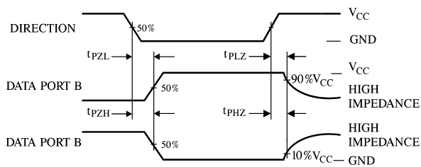
Figure 6. Switching Waveforms
