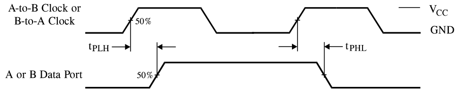
Figure 1. Switching Waveforms
