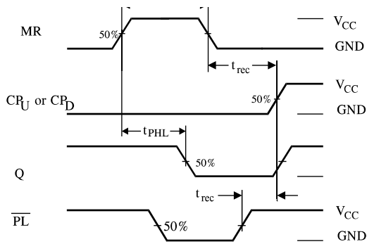
Figure 5. Switching Waveforms
