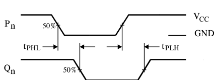
Figure 3. Switching Waveforms
