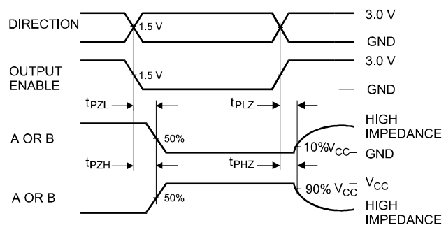
Figure 2. Switching Waveforms
