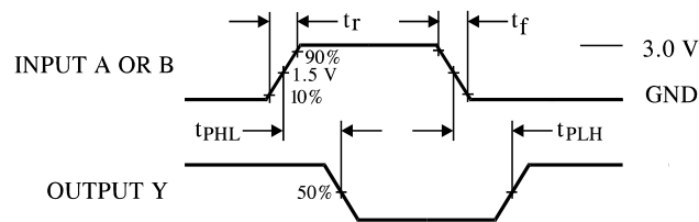
Figure 1. Switching Waveforms
