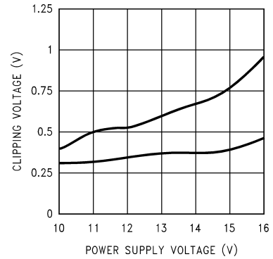
Clipping Voltage vs Power Supply Voltage
