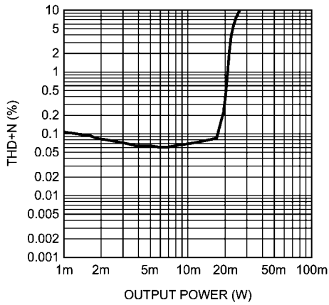
Headphone THD+N vs Output Power AV_{DD} = 5V , OCL 1.2V, 12dB DAC f_{OUT} = 1kHz , 32\Omega
