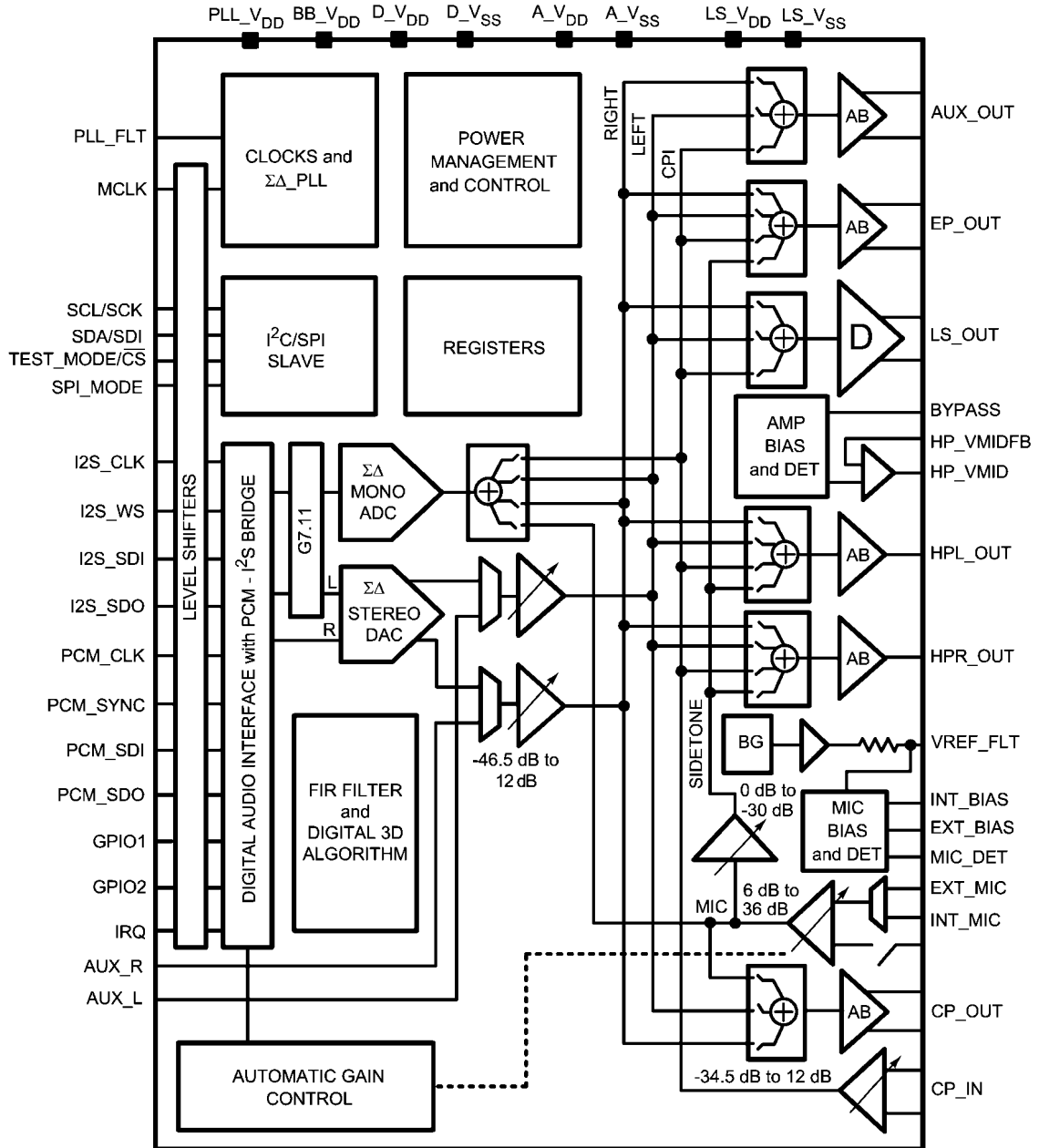
FIGURE 1. Conceptual Schematic
