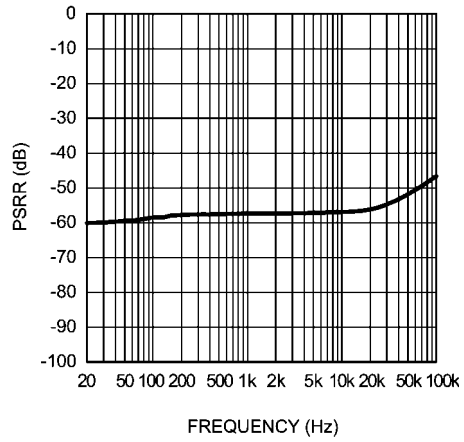
Headphone PSRR vs Frequency V_{DD} = 5V , 0dB AUX, SE (AUX inputs terminated)
