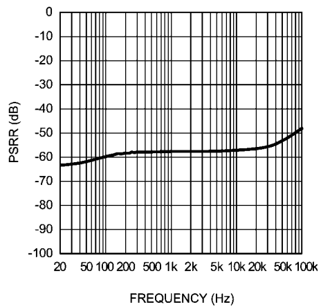
Headphone PSRR vs Frequency V_{DD} = 5V , 0dB DAC, SE (DAC input selected)
