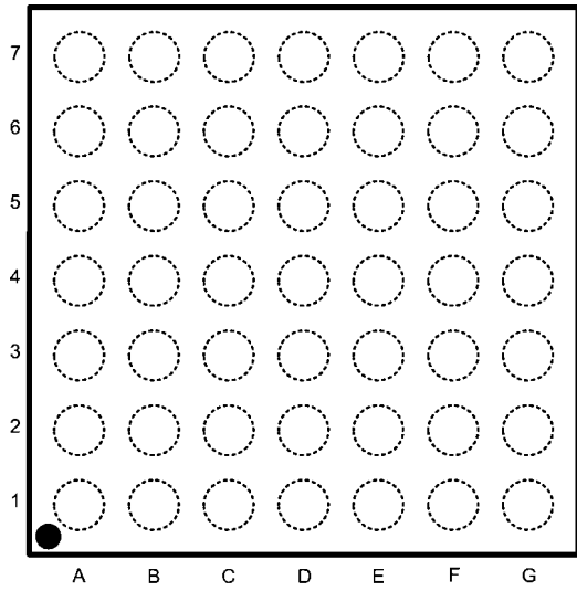
Top View (Bump Side Down) Order Number LM49370RL See NS Package Number RLA49UUA
