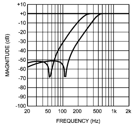
MONO ADC HPF Frequency Response f_s = 16\text{kHz} , 36dB MIC (from left to right: HPF_MODE '00', '10', '01')
