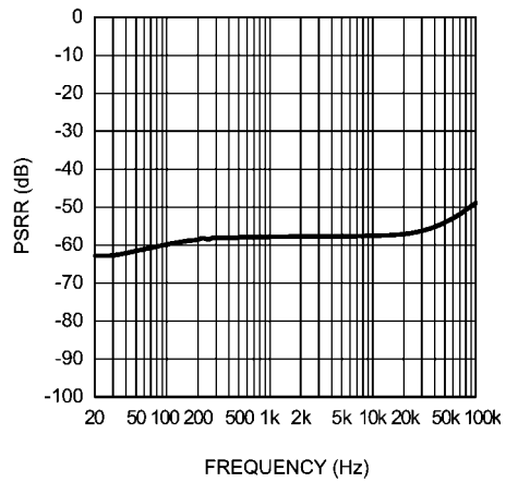
Headphone PSRR vs Frequency V_{DD} = 5V , 0dB CPI, SE (CPI input terminated)
