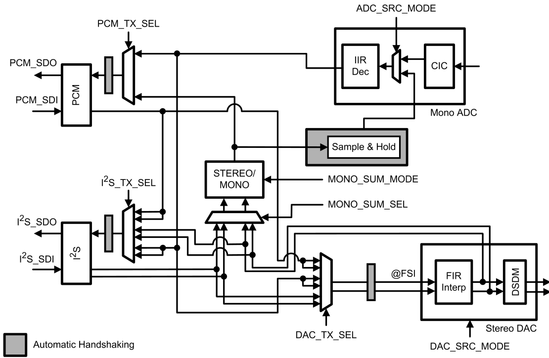
FIGURE 14. I2S to PCM Bridge
