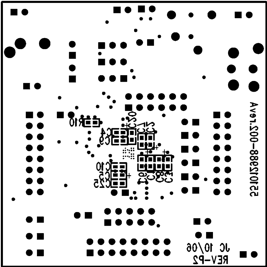
Bottom Silkscreen
