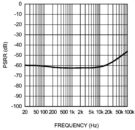
Headphone PSRR vs Frequency V_{DD} = 3.3V , 0dB AUX, SE (AUX inputs terminated)
