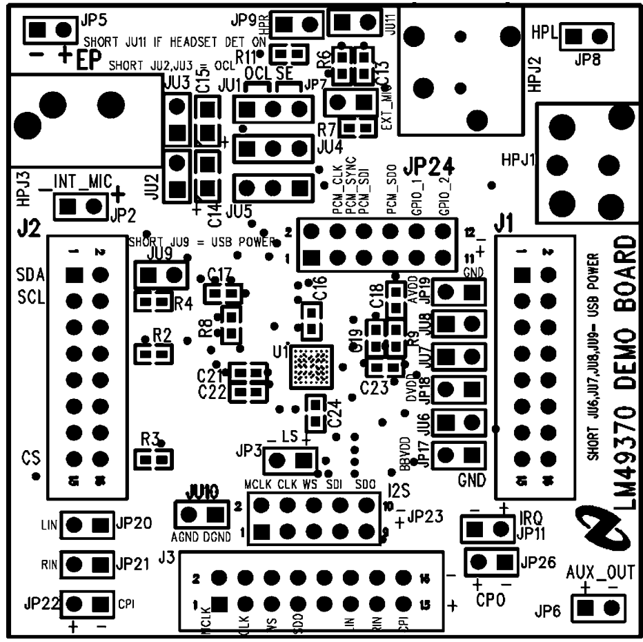
Top Silkscreen
