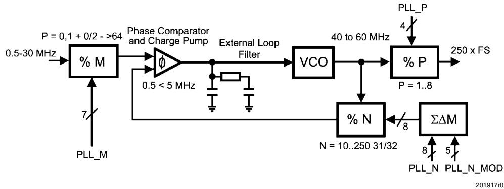
FIGURE 7. PLL Overview
