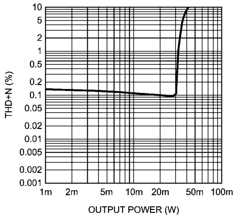
Headphone THD+N vs Output Power AV_{DD} = 5V, OCL 1.5V, 12dB AUX f_{OUT} = 1kHz, 32\Omega
