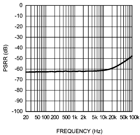
Headphone PSRR vs Frequency V_{DD} = 3.3V , 0dB DAC, SE (DAC input selected)
