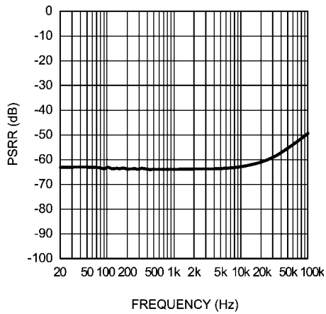
Headphone PSRR vs Frequency V_{DD} = 3.3V , 0dB CPI, SE (CPI input terminated)
