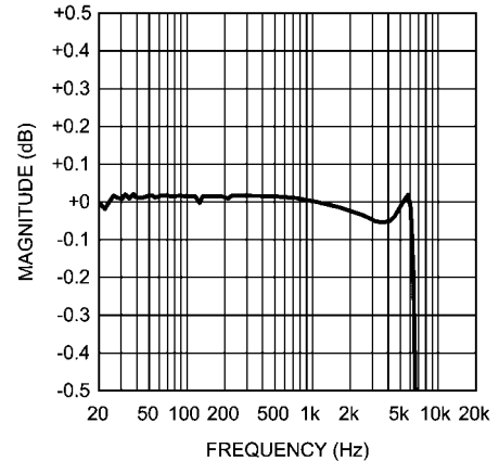
MONO ADC Frequency Response Zoom f_s = 16\text{kHz} , 6dB MIC
