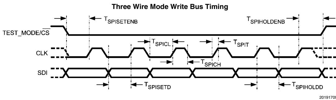
FIGURE 5. SPI Timing
