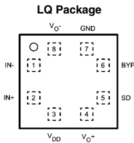
Top View Order Number LM4923LQ See NS Package Number LQB08A
