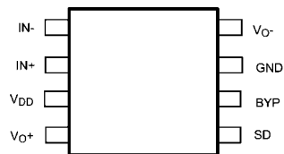
200713a1 Top View See Order Number LM4923MM See NS Package Number MUA08A
