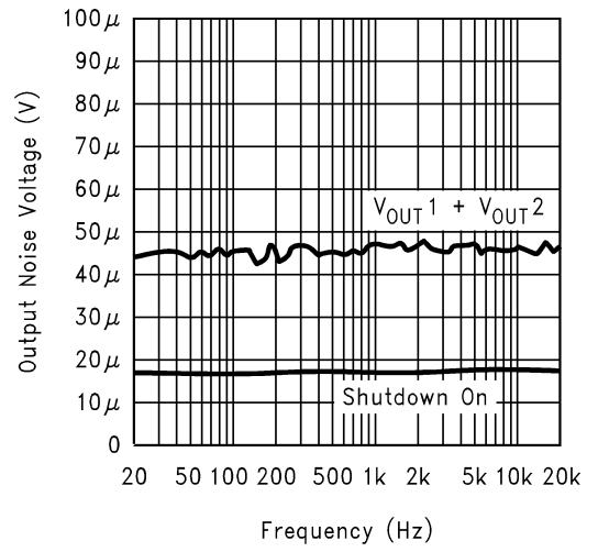
Noise Floor
