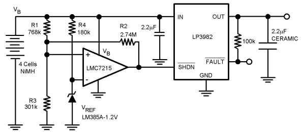
FIGURE 7. Minimum Battery Detector that Disconnects the Load Via the SHDN Pin of the LM4801
