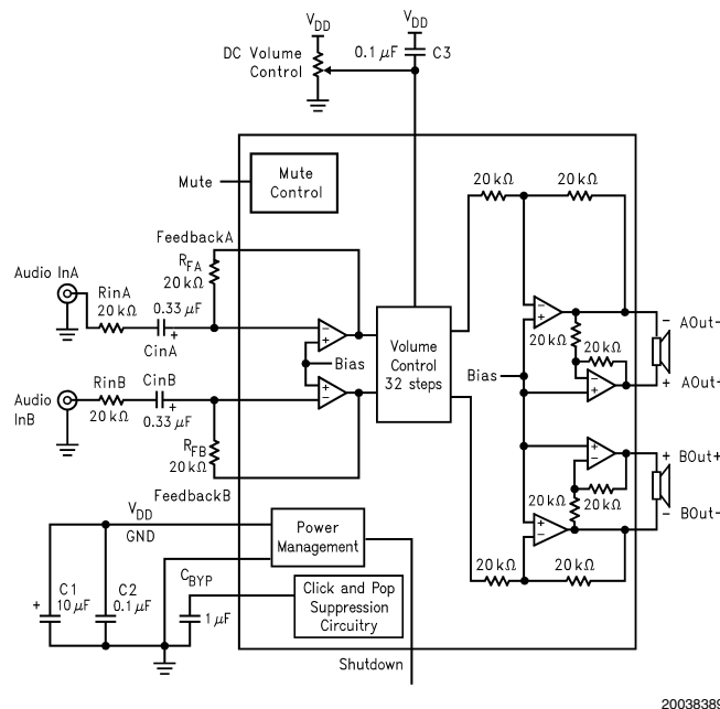
FIGURE 1. LM4843 Block Diagram
