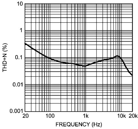
THD+N vs Frequency V_{DD} = 3.6V, R_L = 4\Omega, P_O = 250mW/channel A_V = 6dB
