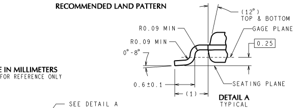
DETAIL A TYPICAL
