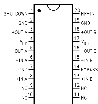
Top View Order Number LM4863MT See NS Package Number MTC20 for TSSOP
