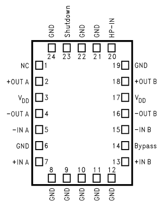
Top View Order Number LM4863LQ See NS Package Number LQA24A for Exposed-DAP LLP
