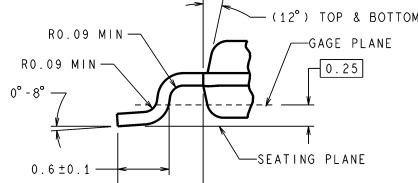
DETAIL A TYPICAL
