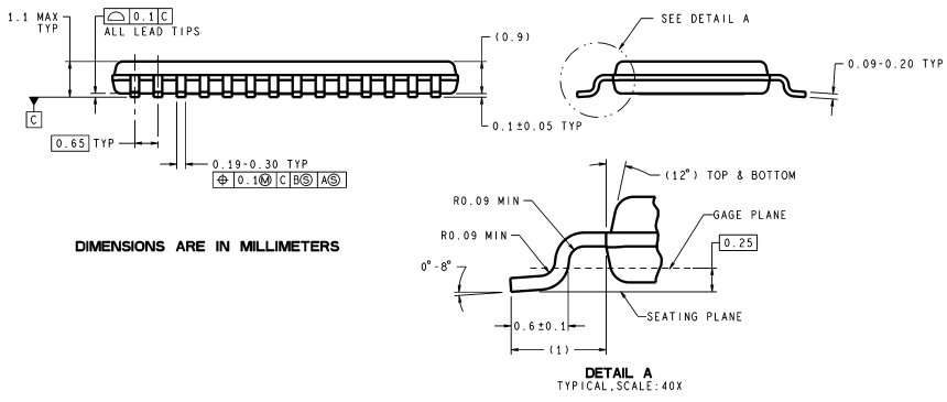
Exposed-DAP TSSOP Package Order Number LM4835MTE NS Package Number MXA28A for Exposed-DAP TSSOP
