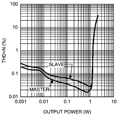
FIGURE 3. THD+N vs Output Power
