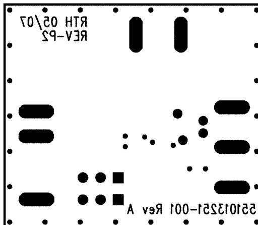
FIGURE 14. Bottom Silkscreen
