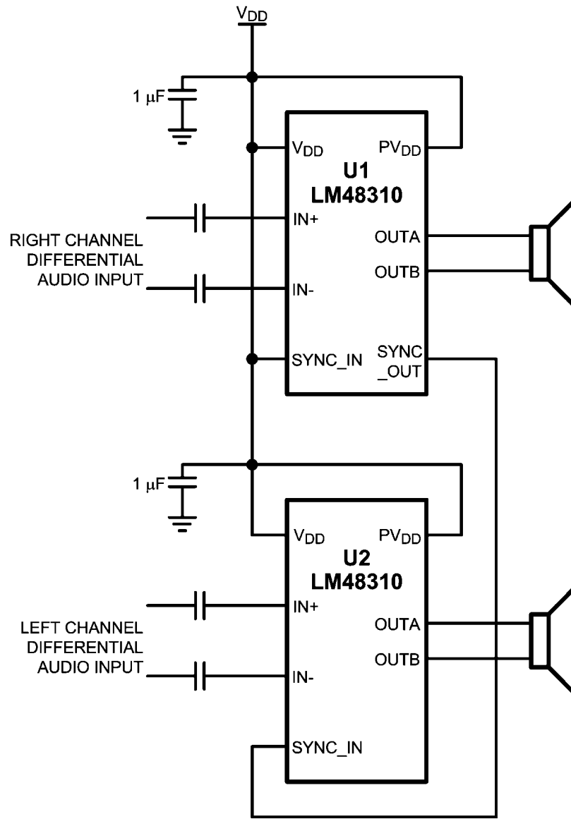
FIGURE 2. Cascaded LM48310
