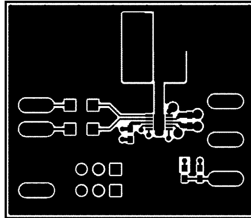
FIGURE 10. Top Layer
